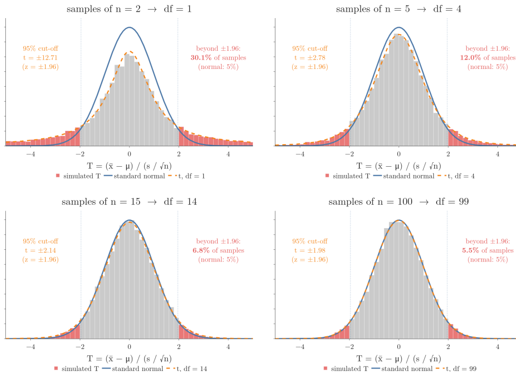
Figure 4: Simulated T values for samples of n = 2 to 100 (histogram) against the standard normal (blue) and the t-curve with df = n - 1 (orange); the share beyond \pm 1.96 falls from 30% towards 5%
