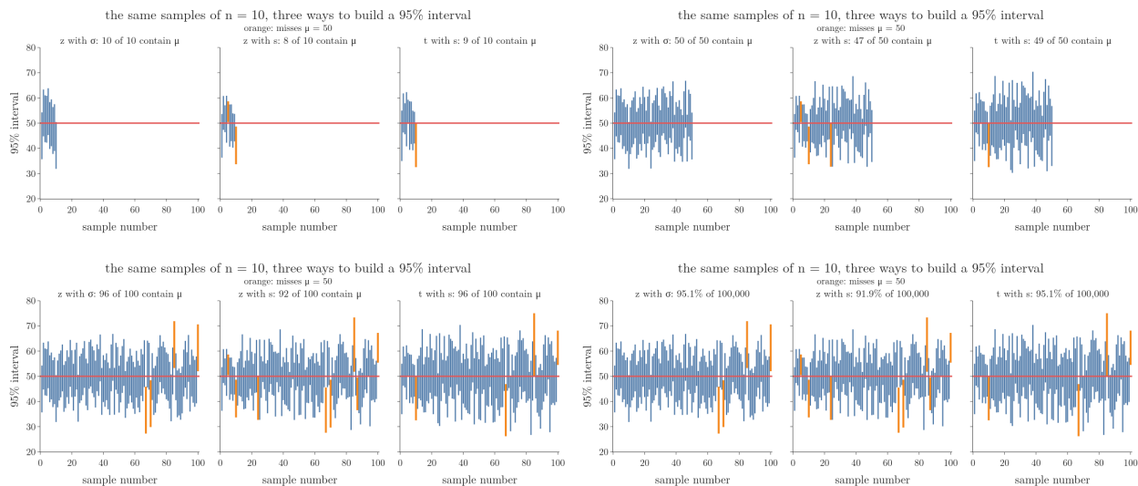
Figure 2: The same samples of n = 10 with three 95% intervals each: z with the true sigma, z with s , and t with s ; misses in orange, running counts in the titles, coverage over 100,000 samples in the last frame (idea after Khan Academy, “Simulation showing value of t statistic”)
