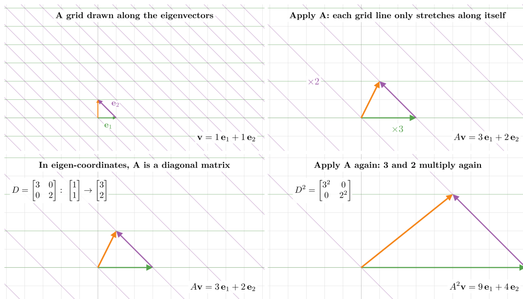
Figure 7: A grid drawn along the eigenvectors \mathbf{e}_1 = [1, 0] and \mathbf{e}_2 = [-1, 1] ; applying A only stretches its lines, so \mathbf{v} = 1\mathbf{e}_1 + 1\mathbf{e}_2 lands on 3\mathbf{e}_1 + 2\mathbf{e}_2 , then 9\mathbf{e}_1 + 4\mathbf{e}_2
