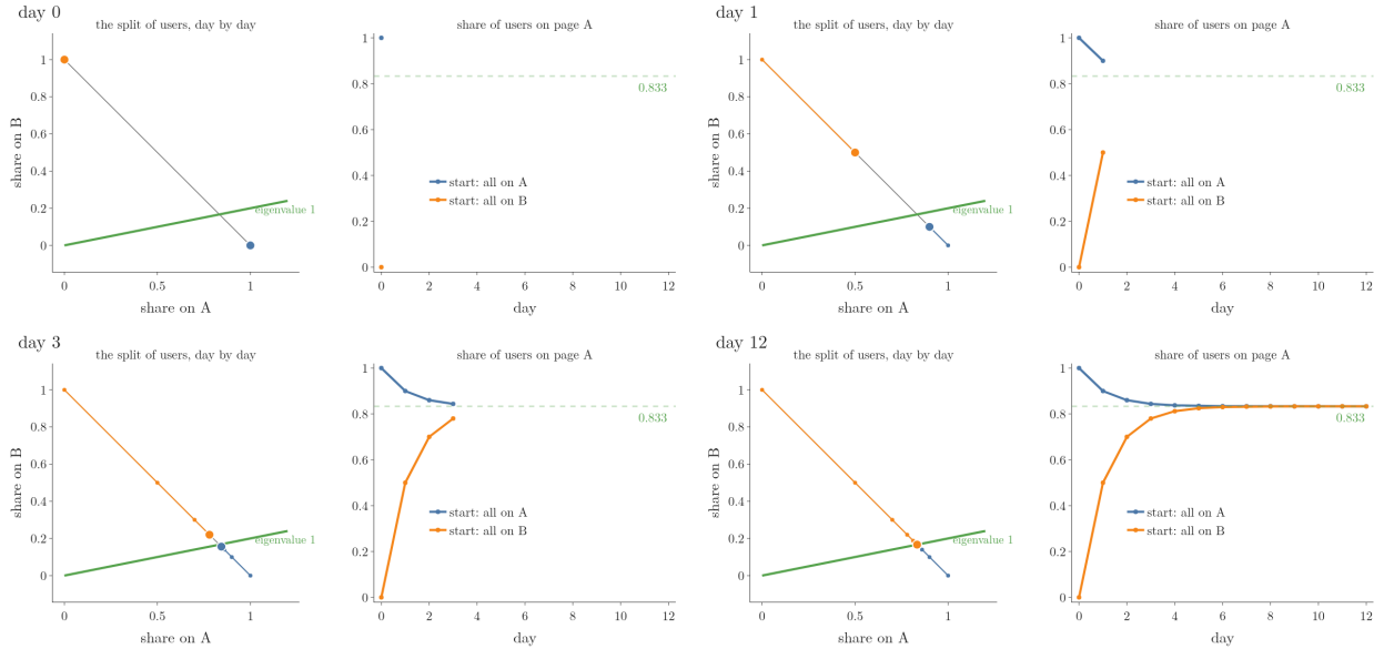
Figure 8: Power iteration with the one-day matrix T . Left: each day's split of users as a point; both starting splits slide onto the green eigenvector of eigenvalue 1. Right: the share of users on page A settles at 0.833 from either start.
