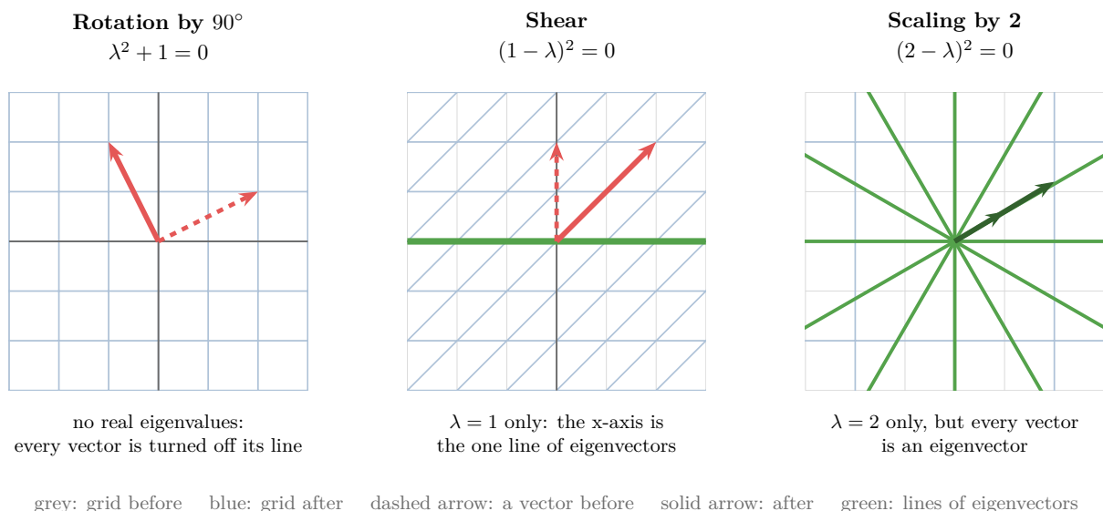
Figure 6: Three transformations with very different eigenvectors
