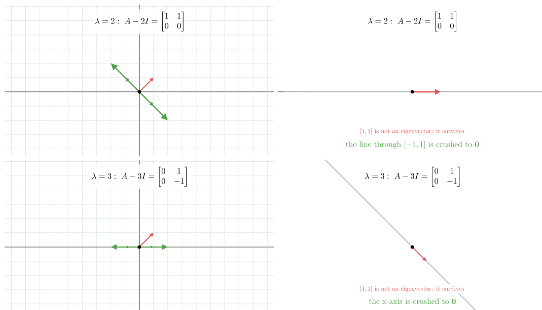
Figure 5: The plane moves under A - 2I (top) and A - 3I (bottom). Green: vectors on the eigenvector line, sent to the origin. Red: [1, 1] , which is not an eigenvector and survives.
