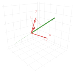
Figure 3: A rotation about the axis through [1, 1, 1] , from 0 to 120 degrees. Red: the basis vectors x , y and z , turned off their lines. Green: the axis, an eigenvector with eigenvalue 1, which never moves.
