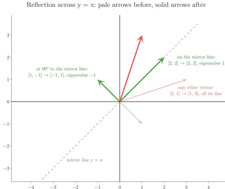
Figure 2: Reflection across the line y = x . Green: the two eigenvector lines, one kept in place (eigenvalue 1) and one flipped (eigenvalue -1 ). Red: [3, 1] is knocked off its line. Example after Khan Academy, “Introduction to eigenvalues and eigenvectors”, with our own mirror line.
