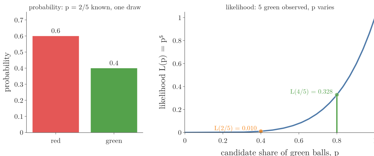
Figure 3: The bag read both ways. Left, probability: with p = 2/5 known, a draw is red with probability 0.6 and green with 0.4. Right, likelihood: with five green draws observed, L(p) = p^5 for every share p of green balls; L(2/5) = 0.010 and L(4/5) = 0.328 .
