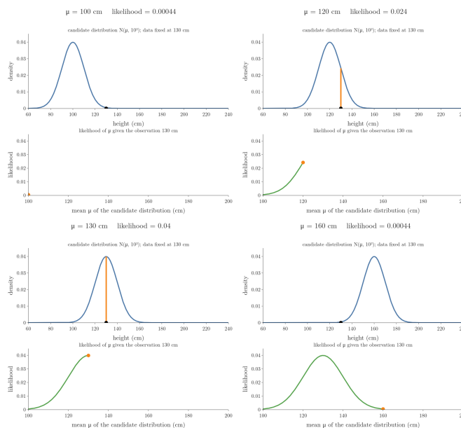
Figure 4: One person measured at 130 cm. Top: the candidate curve N(\mu, 10^2) slides; the orange bar is its height at 130. Bottom: those heights against \mu , the likelihood function, highest at \mu = 130
