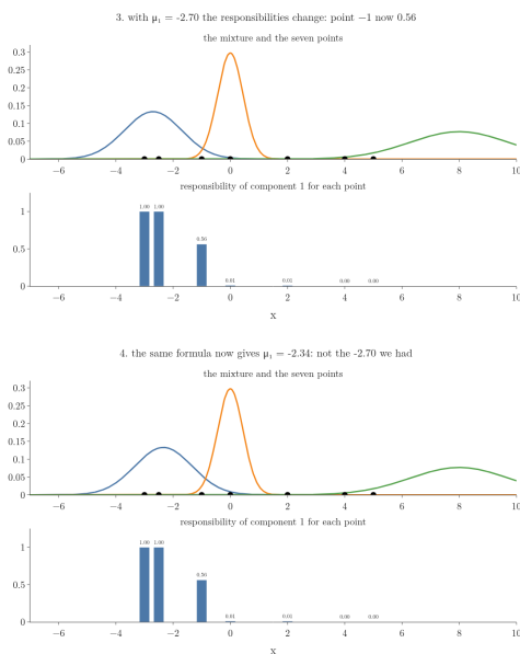
Figure 7: The circular dependence on the seven points. 1: the starting mixture. 2: the slope-zero formula moves \mu_1 from -4 to -2.70 . 3: with the new \mu_1 the responsibilities change; point -1 now belongs 0.56 to component 1. 4: the same formula now gives -2.34 .
