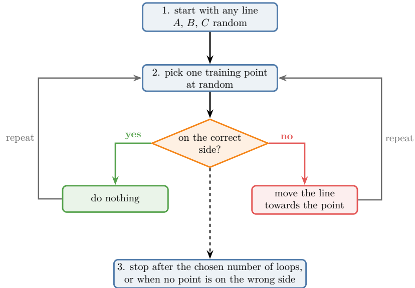
Figure 4: The perceptron trick as a loop: start with any line, pick a random training point, leave the line alone if the point is on the correct side, otherwise move the line towards it; repeat until the chosen number of loops is done or no point is wrong.
