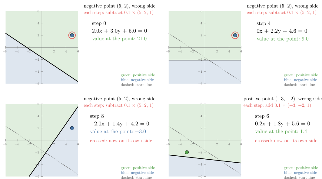
Figure 7: The perceptron trick in small steps, learning rate 0.1. First, the negative point (5, 2) sits on the positive (green) side; each step subtracts 0.1 \times (5, 2, 1) from the coefficients, its value falls by 3 (21, 18, 15, ...), and at step 8 the point is on the negative side. Then the positive point (-3, -2); each step adds 0.1 \times (-3, -2, 1) , its value rises by 1.4 from -7, and it crosses at step 6. The dashed line is the start line 2x + 3y + 5 = 0
