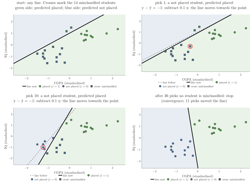
Figure 5: The perceptron trick on 24 students, learning rate 0.1. Each frame picks one student (red ring). Correct side: the line stays. Wrong side (cross): the line moves towards the student; the dashed line is the line before the move. The run stops after 36 picks, when no student is misclassified.
