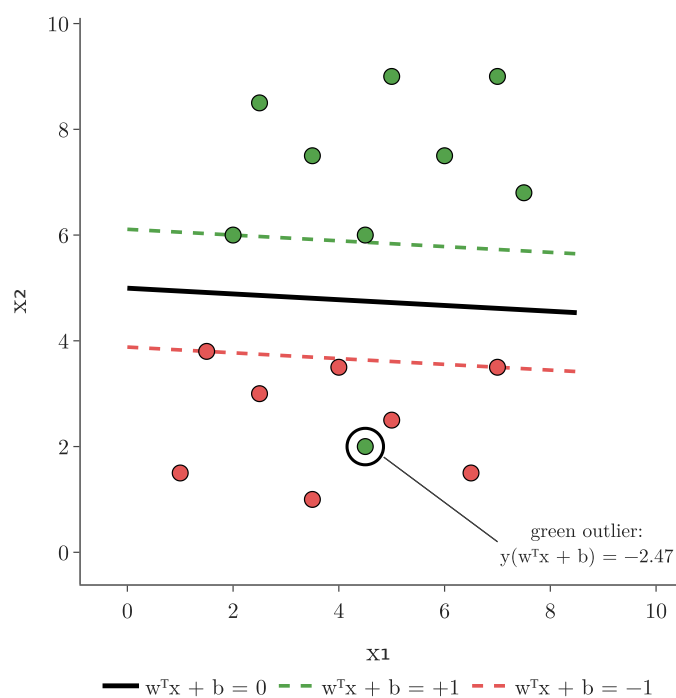
Figure 7: A single green outlier among the red points breaks the constraints of every line
