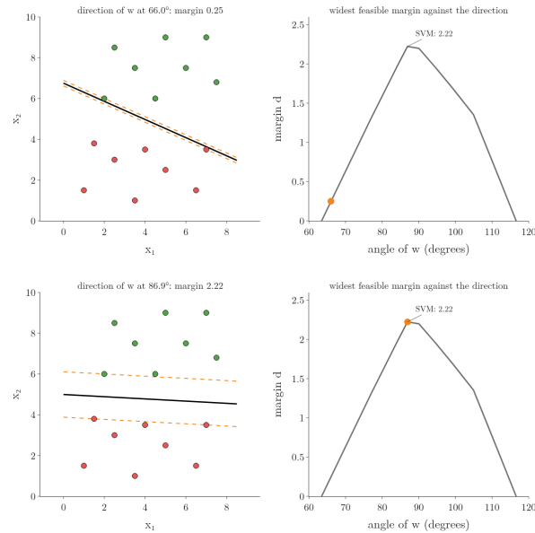
Figure 6: The optimisation as a search over directions of w , on the 16 points of the SVM intuition Note. Left: for one direction, the line in the middle of the widest gap it allows (dashed: \pi^+ and \pi^- ). Right: that widest margin against the angle of w ; the maximum, 2.22, is at the direction of the SVM's w .
