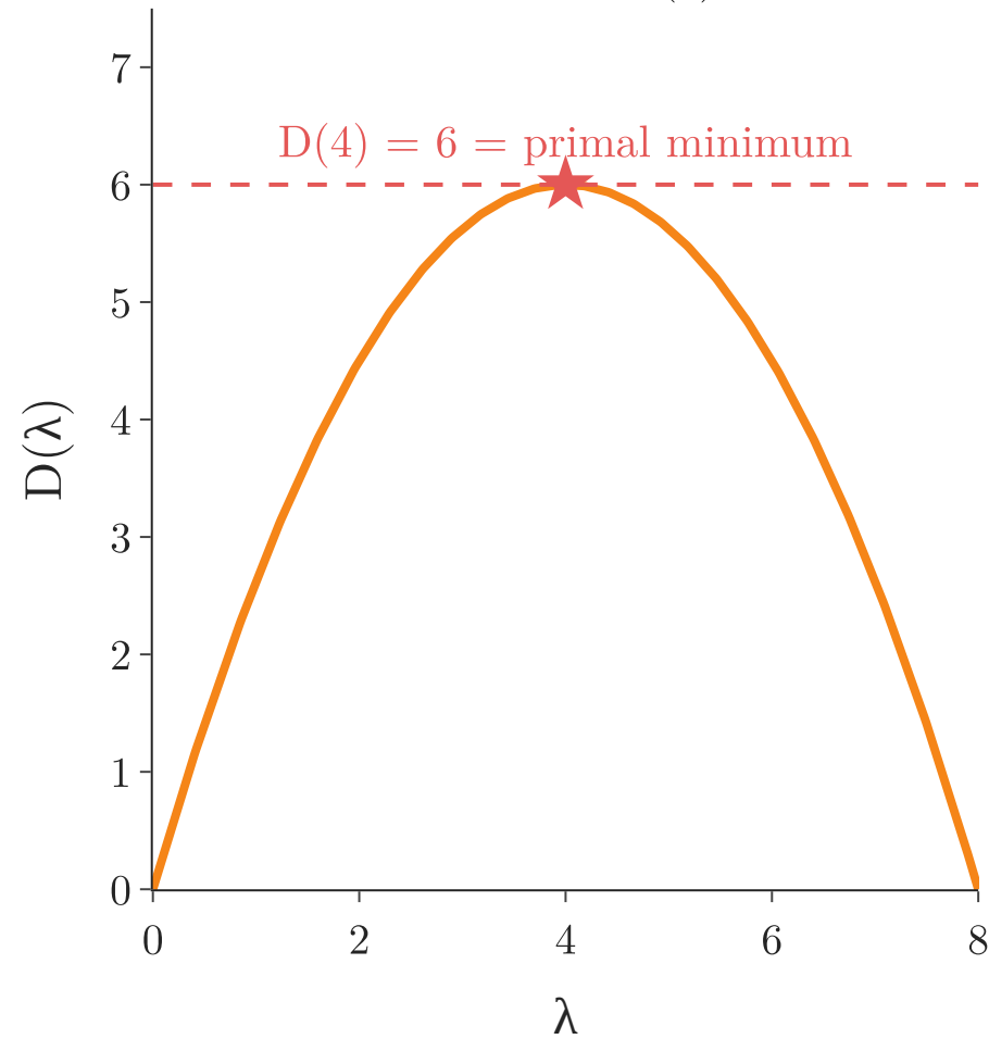
dual: \max D(\lambda)
