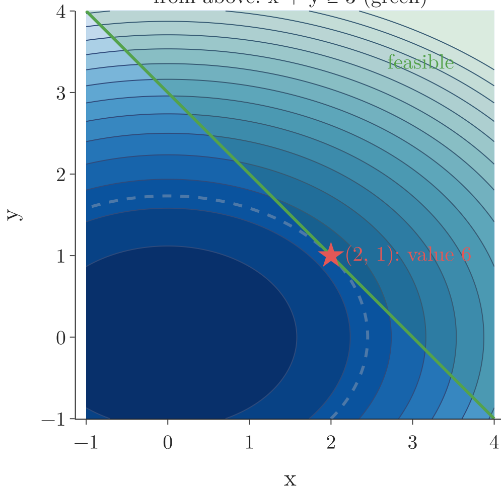
from above: x + y \geq 3 (green)
