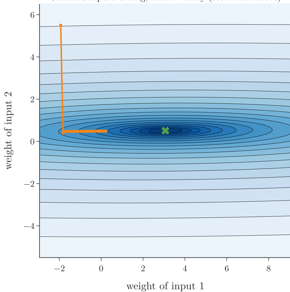
Unscaled inputs: a long, narrow valley (seen from above)
