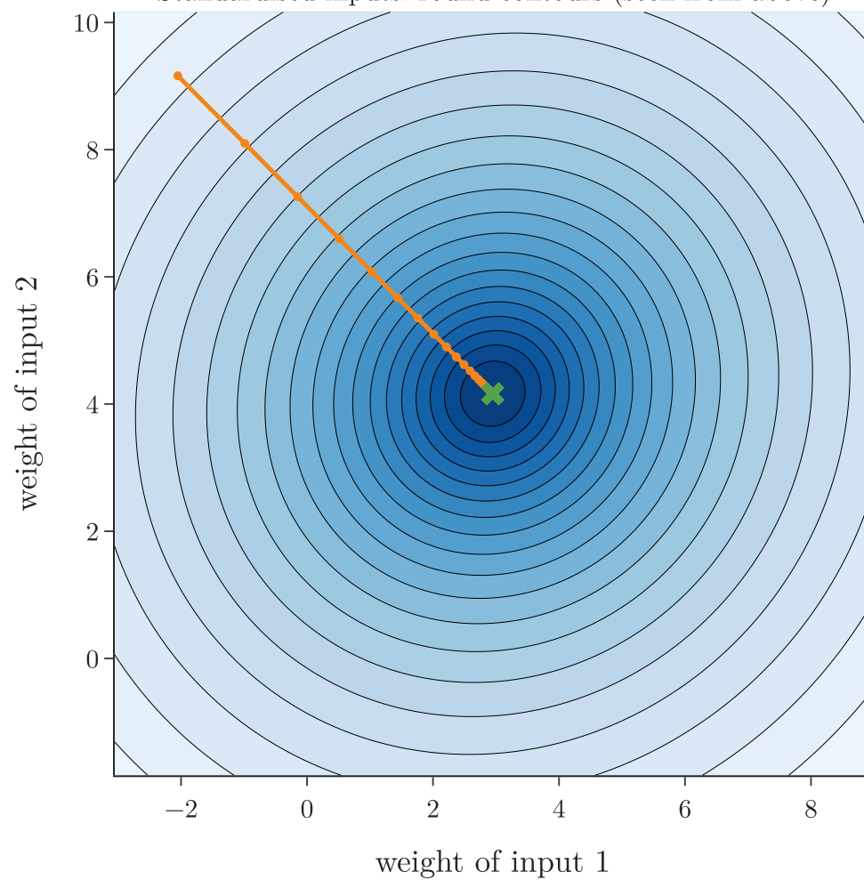
Standardised inputs: round contours (seen from above)
