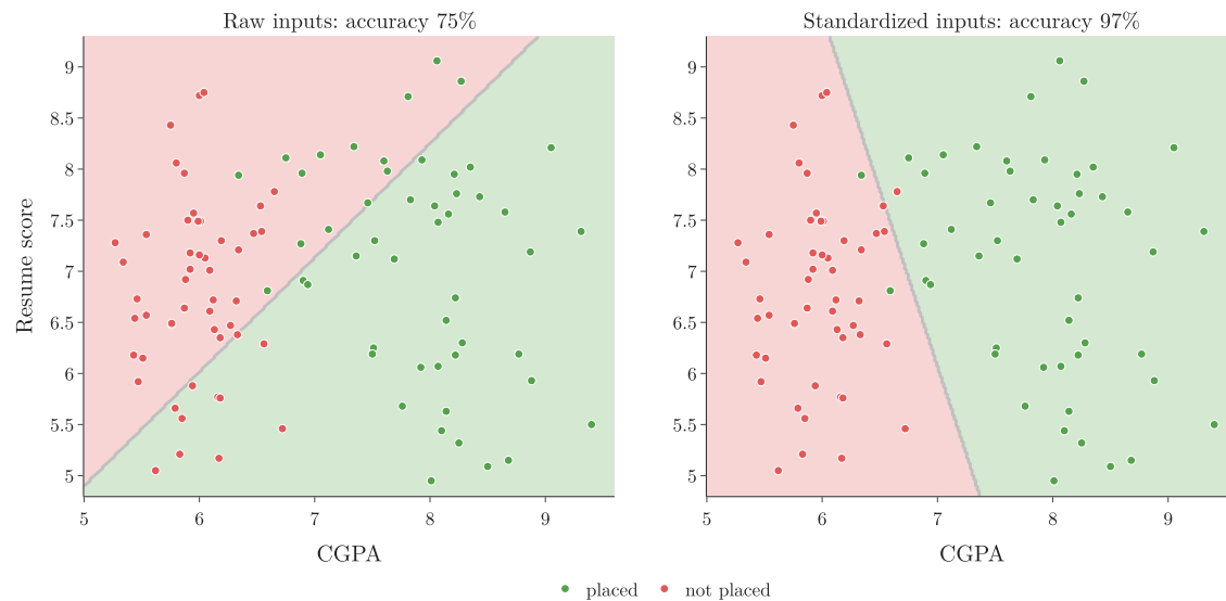
Figure 8: The perceptron’s line and its two regions, before and after standardizing the inputs
