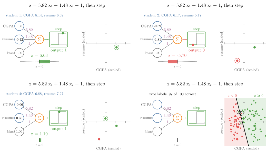
Figure 3: Prediction with a trained perceptron, z = 5.82x_1 + 1.48x_2 + 1 on standardized CGPA and resume score. For each student the inputs flow in, z fills a bar (green if positive, red if negative), the step function fires 1 or 0, and the student lands on the plane in that colour. At the end all 100 students appear with the line z = 0 between the two regions
