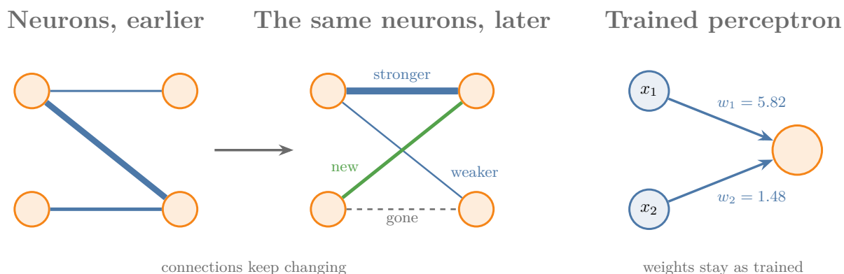
Figure 5: Neuroplasticity: connections between neurons get stronger, get weaker, vanish and appear over time; the weights of a trained perceptron stay fixed
