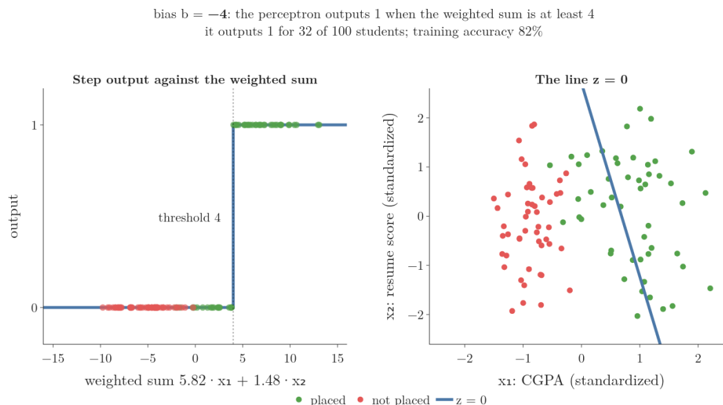
Figure 2: The bias as a threshold. Left: the step output against the weighted sum; the jump sits at -b . Right: the same perceptron on the input plane; the line z = 0 moves sideways without turning. The bias goes from 4 down to -4 .
