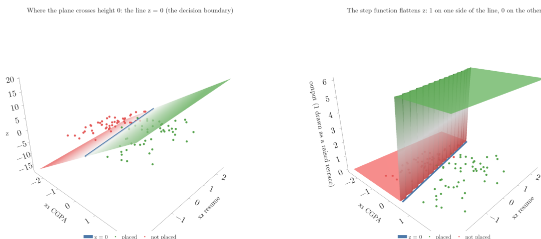
Figure 7: The perceptron of section 8 in 3D. First z is a tilted plane above the students; it crosses height 0 along the line z = 0 ; then the step function turns z into two flat terraces, 1 and 0.
