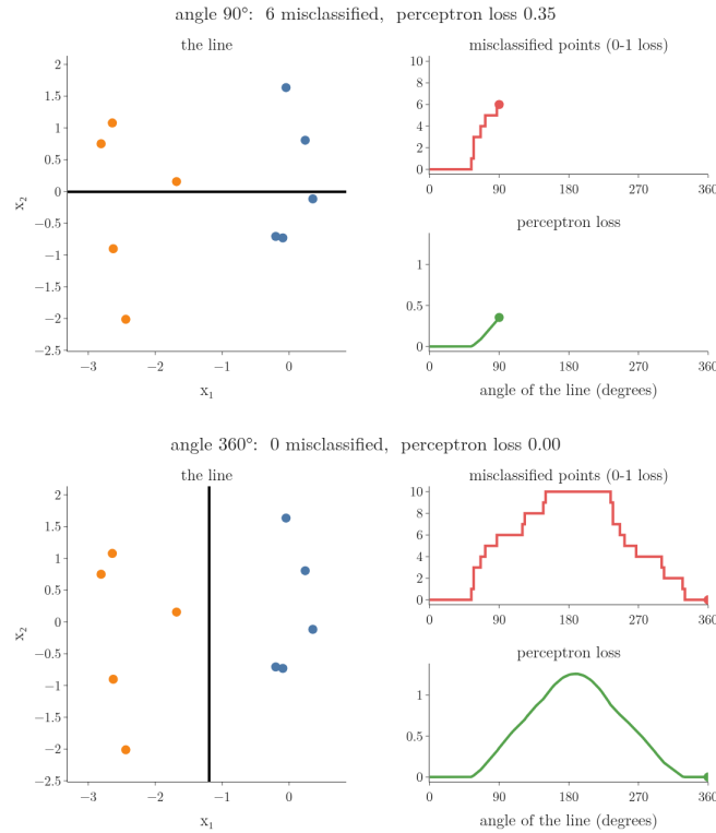
Figure 5: A line turning through 360 degrees over 10 points. Top right: the number of misclassified points (0-1 loss). Bottom right: the perceptron loss, the average of the values of the misclassified points
