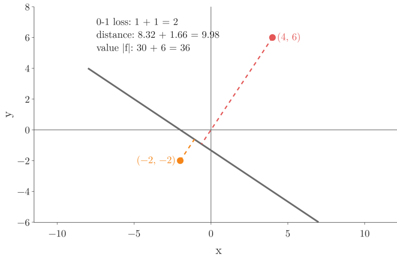
Figure 4: The line 2x + 3y + 4 = 0 and its two misclassified points, with their perpendicular distances (dashed) and the three candidate losses
