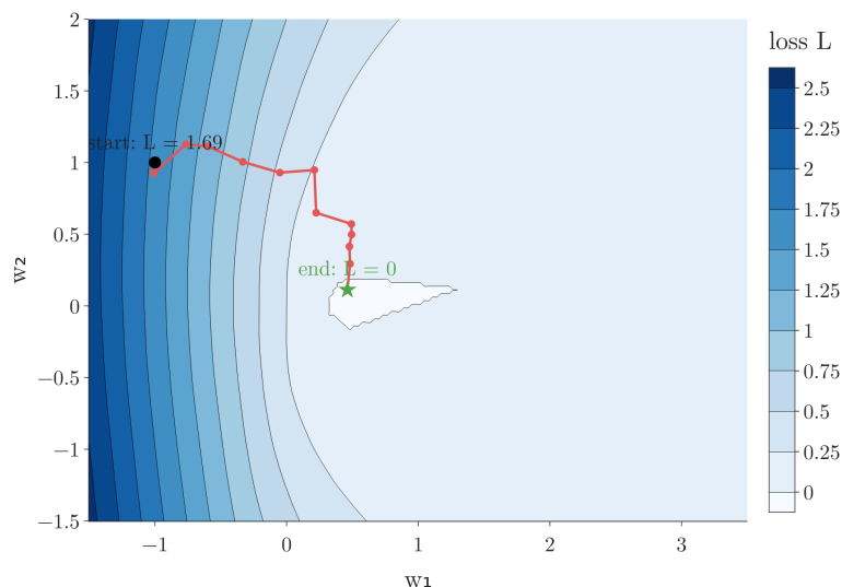
Figure 3: The perceptron loss of Section 6 for the 100 points of Figure 1, over w_1 and w_2 (with b held at its final value 0.5), and the path of the 12 updates of Figure 1
