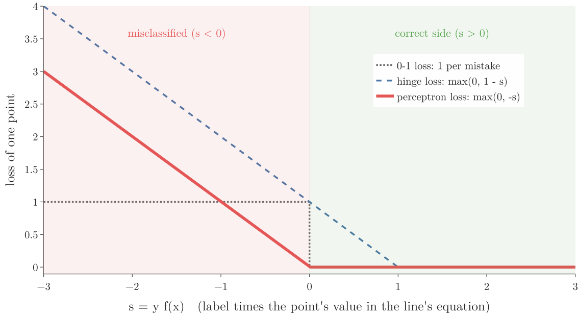
Figure 7: The loss of one point against s = y f(x)
