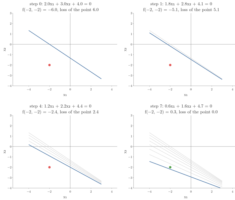
Figure 8: The same step repeated on the point (-2, -2) : each step raises f(-2, -2) by 0.1 \times ((-2)^2 + (-2)^2 + 1) = 0.9 , until the point crosses the line after 7 steps
