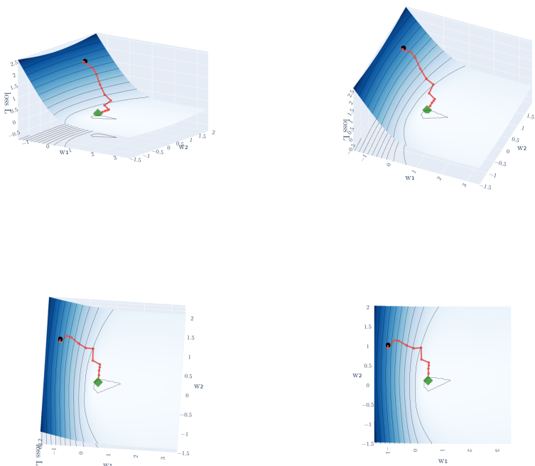
Figure 2: The same loss surface: it slopes down from the dark left edge to a flat floor where L = 0 . The camera tilts from a side view to the top view; the black lines join points at the same height. The red path is the 12 updates of Figure 1 (black dot: start, green diamond: end)
