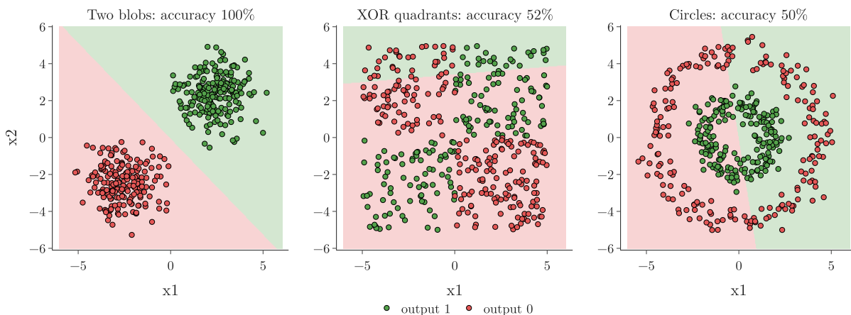
Figure 4: One sigmoid neuron on linearly separable, XOR-shaped and circular data
