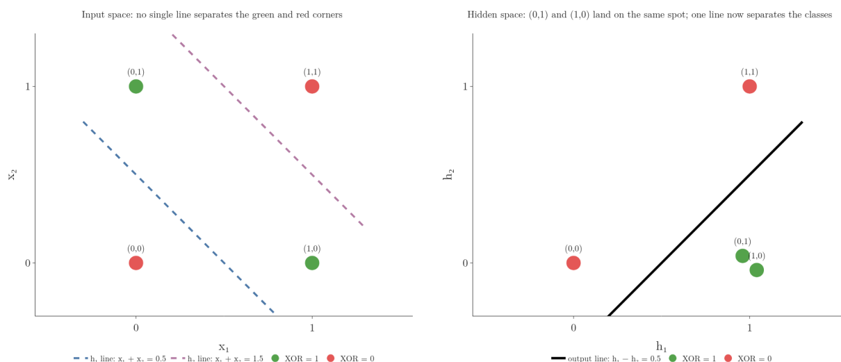
Figure 5: The four XOR observations moved by two hidden perceptrons, h_1 = \text{step}(x_1 + x_2 - 0.5) and h_2 = \text{step}(x_1 + x_2 - 1.5) . Left: the input square with the two hidden lines. Right: the new positions, where one line separates the classes.
