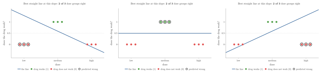
Figure 3: A drug that works only at a medium dose. A straight line is turned through every slope and placed at its best height; a black ring marks a patient predicted wrong. The line never gets more than 2 of the 3 dose groups right. Idea after StatQuest, “The Essential Main Ideas of Neural Networks”.
