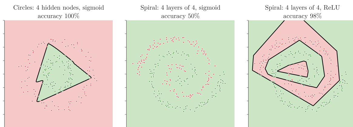
Figure 12: MLPs trained on two circles and on two spirals
