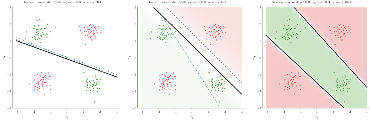
Figure 11: The 2-2-1 network of Figure 10 during gradient descent. Shading: the output node’s probability of class 1 (green); black: its 0.5 decision boundary; dashed and dotted: the two hidden nodes’ lines.
