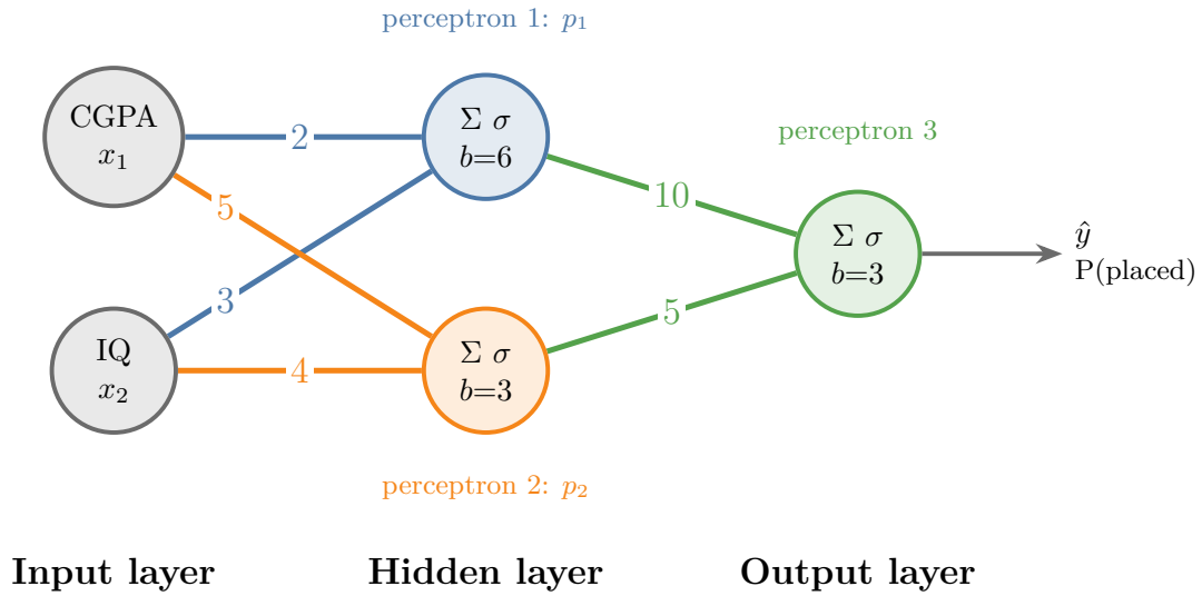
Figure 7: The model of Section 3.3 as a network: perceptrons 1 and 2 read CGPA and IQ; perceptron 3 combines their outputs
