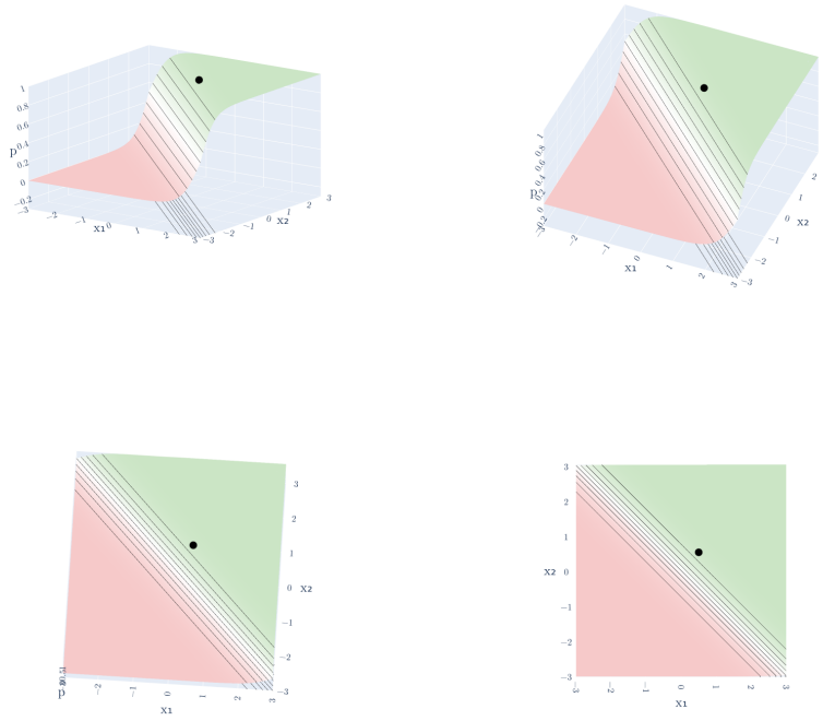
Figure 2: The surface p = \sigma(3x_1 + 3x_2) : a smooth ramp from 0 up to 1. The camera tilts from a side view to the top view; the black lines join points at the same height. Black dot: the point (0.5, 0.5)
