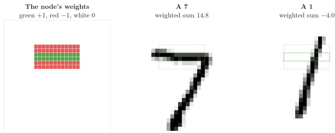
Figure 9: One hidden node as an edge detector. Left: its weights, set by hand: +1 on a horizontal strip, -1 just above and below, 0 elsewhere. Middle and right: a 7 and a 1 from the MNIST digits, with the strip outlined. Idea after 3Blue1Brown, “But what is a neural network?”.
