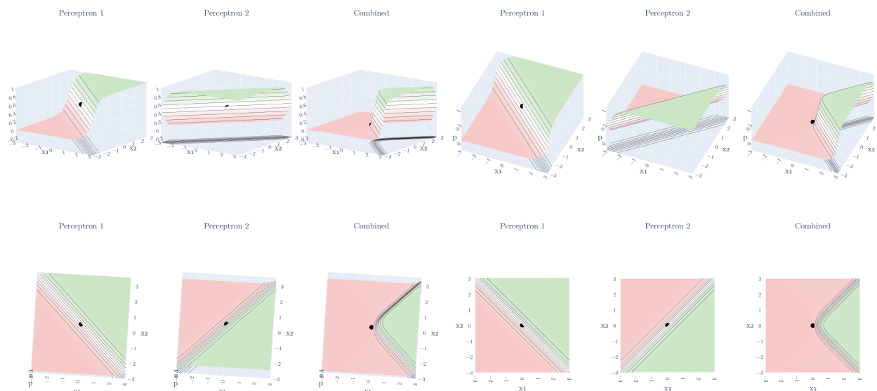
Figure 4: The surfaces of perceptron 1, perceptron 2 and their combination. The camera tilts from a side view to the top view; the black lines join points at the same height. Black dot: the point (0,0)
