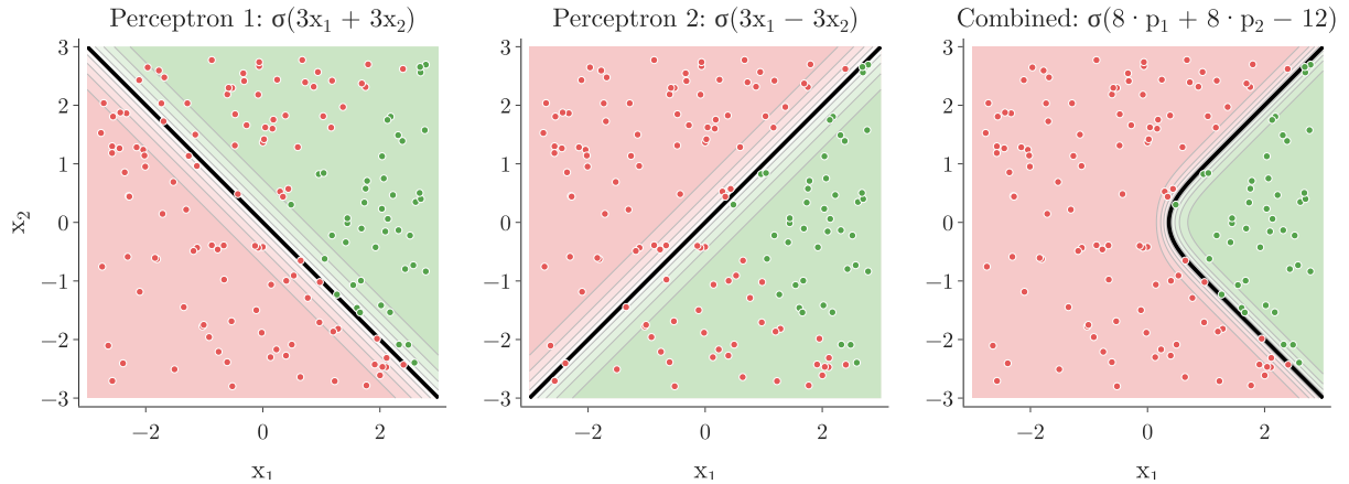
Figure 5: Two perceptrons and their combination. Shading: probability of green; black: the 0.5 boundary. The weights are our own, chosen to show the effect.
