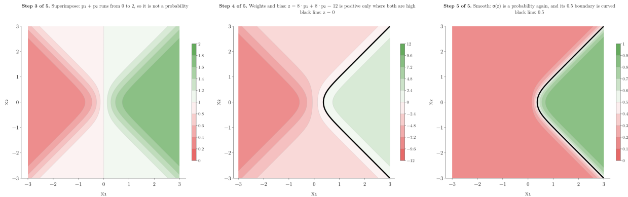
Figure 6: Superimpose, then smooth. Frames: perceptron 1's map; perceptron 2's map; their plain sum, which runs from 0 to 2; the weighted sum with the bias, 8p_1 + 8p_2 - 12 ; and its sigmoid, with the curved 0.5 decision boundary in black
