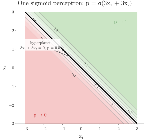
Figure 3: One sigmoid perceptron, p = \sigma(3x_1 + 3x_2) , as a probability map. Thin lines: where p is 0.1, 0.2, ..., 0.9. Thick black line: p = 0.5 , the perceptron's hyperplane.
