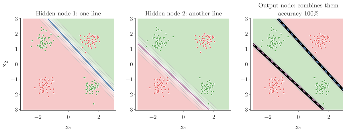
Figure 10: XOR with two hidden nodes. Left and middle: what each hidden node learned, with its line (the 0.5 boundary). Right: the output node's map; its boundary (black) lies on the two hidden lines (dashed).
