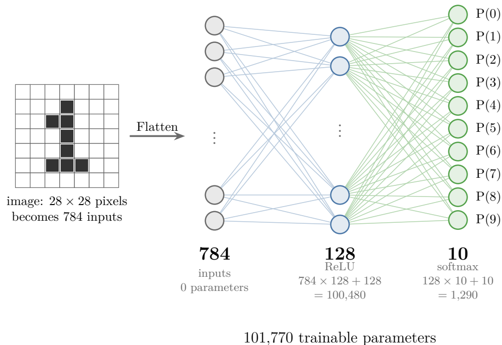
Figure 4: The first MNIST network: the image is flattened into 784 inputs, which feed 128 ReLU nodes and then 10 softmax nodes, one per digit
