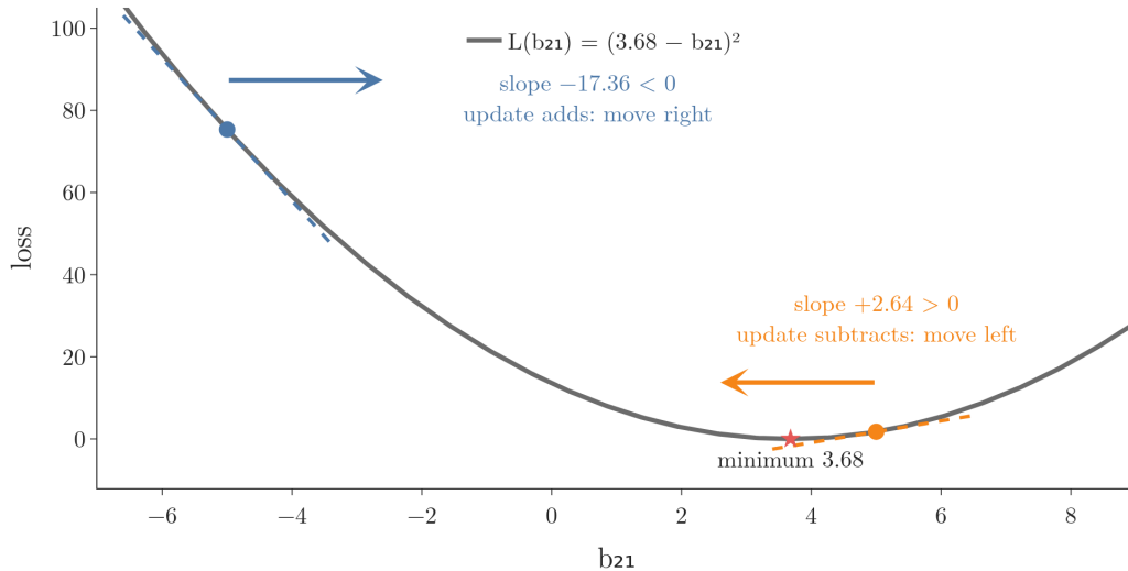
Figure 7: The same loss L(b_{21}) at two points: on the left the slope is negative and the update moves right; on the right it is positive and the update moves left
