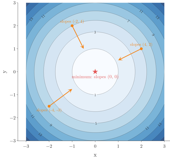
Figure 6: Contours of z = x^2 + y^2 . At three points the arrow is minus the two slopes; only at the star are both slopes zero
