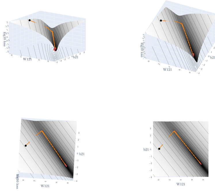
Figure 8: The loss surface of the two knobs W_{21}^1 and b_{21} (height: \log_{10} of the mean loss): a long, narrow valley. The camera tilts from a side view to the top view; the black lines join points at the same height. Orange: the path of Figure 9; black dot: start; red diamond: the lowest point
