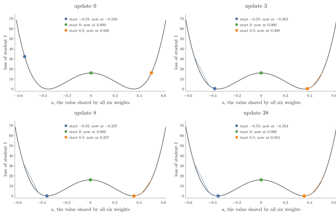
Figure 11: Three runs of gradient descent on L(a) = (4 - 32a^2)^2 , from the starts -0.55 , 0 and 0.5 , with learning rate 0.0003
