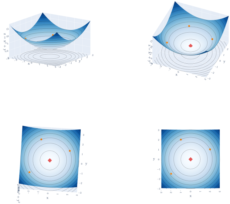
Figure 5: The surface z = x^2 + y^2 , a bowl. The camera tilts from a side view to the top view; the black lines join points at the same height. Orange dots: the three points of Figure 6; red diamond: the minimum
