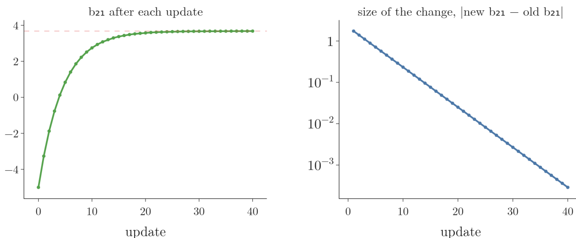
Figure 10: With learning rate 0.1: b_{21} after each update (left) and the size of each change (right, log scale)
