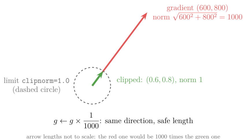
Figure 9: Clipping by norm, on an example gradient of two weights: the gradient of norm 1000 is scaled to norm 1 and keeps its direction
