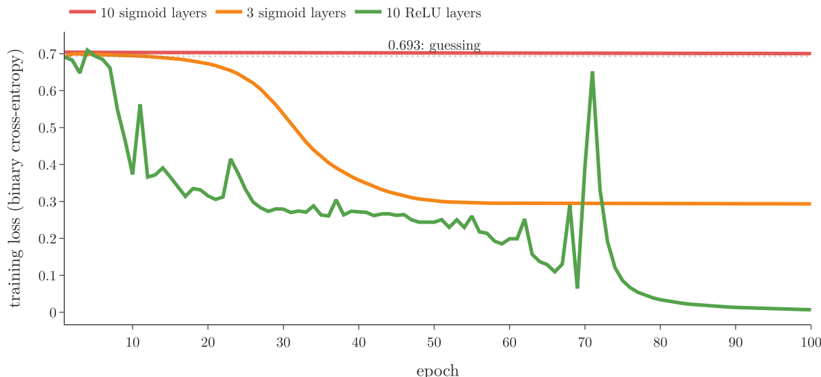
Figure 4: Training loss over 100 epochs: 10 sigmoid layers stay at the guessing level; 3 sigmoid layers and 10 ReLU layers learn
