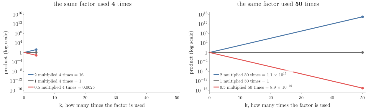
Figure 3: One factor multiplied by itself k times, for k from 1 to 50, on a log scale: 2 (blue), 1 (grey) and 0.5 (red). Idea after StatQuest, “Recurrent Neural Networks (RNNs), Clearly Explained!!!”
