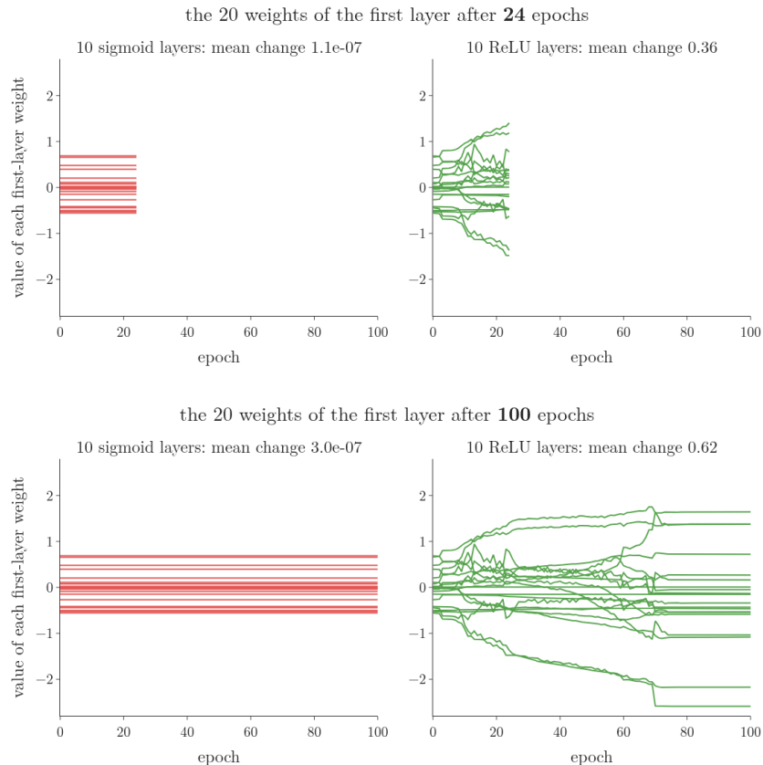
Figure 6: The 20 weights of the first layer, one line each, over the 100 epochs. Left: 10 sigmoid layers. Right: 10 ReLU layers
