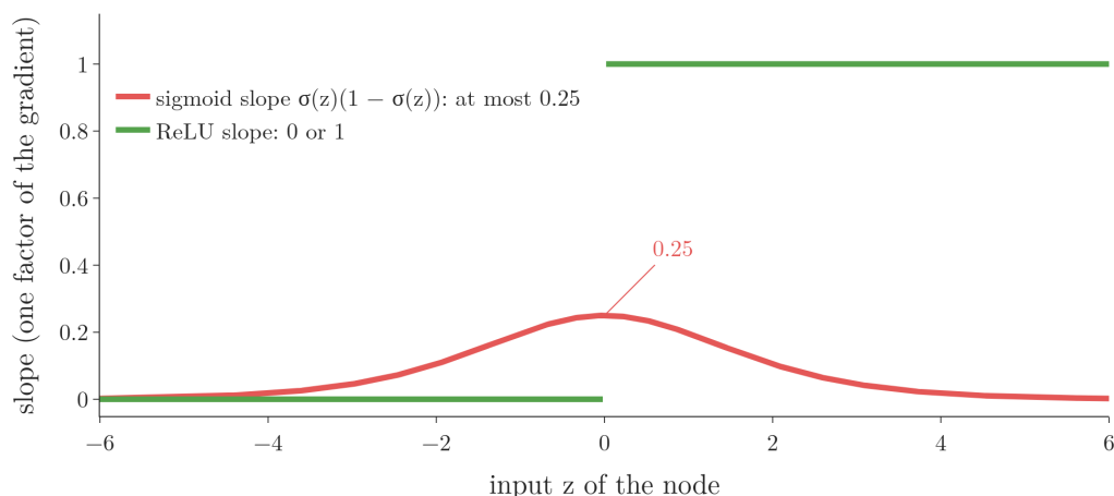
Figure 7: The slope of each activation against its input: sigmoid (red) never exceeds 0.25; ReLU (green) is exactly 0 or 1
