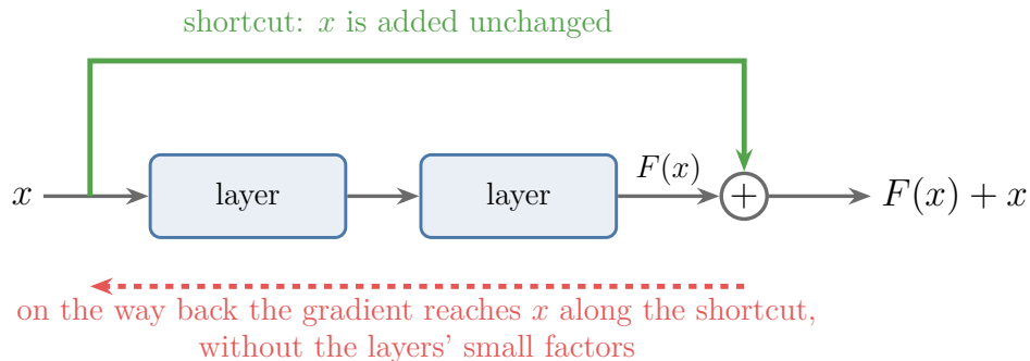
Figure 8: A residual block: the output is the layers' result F(x) plus the input x
