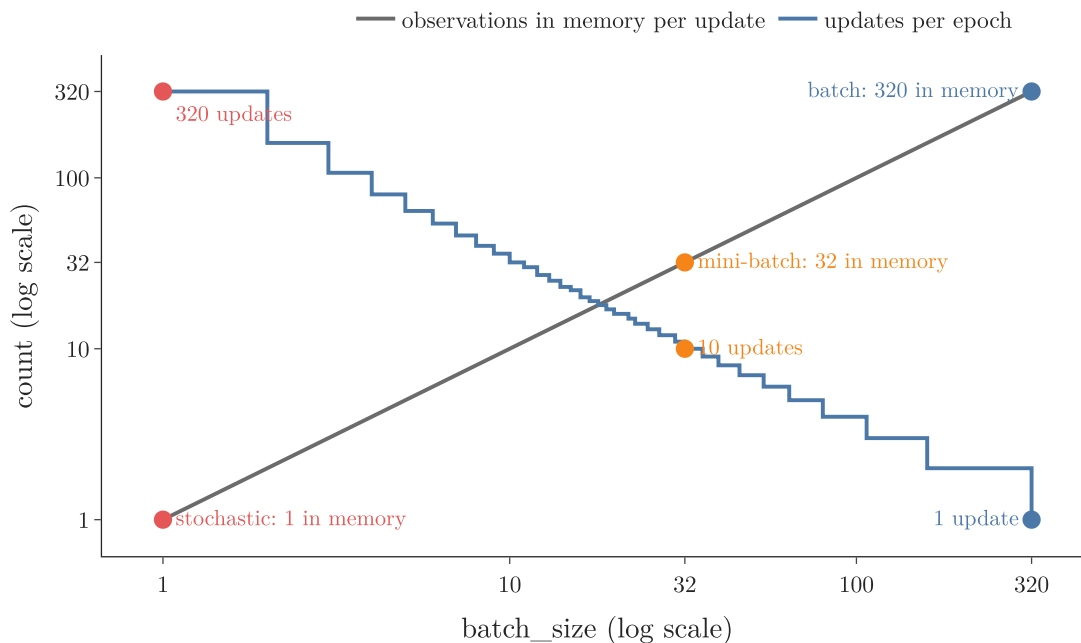
Figure 9: The two costs of batch_size on our 320 training observations (both axes log scale). Grey: observations that must sit in memory for one update. Blue: updates per epoch, \lceil 320/\text{batch size} \rceil .
