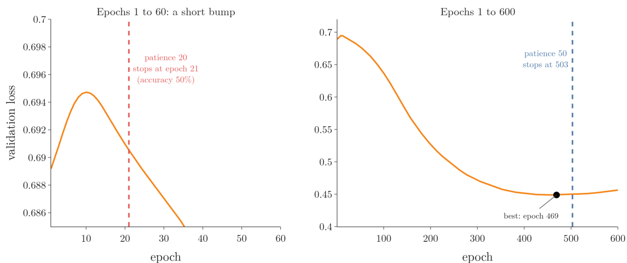
Figure 4: Keras’ stopping rule replayed on the validation loss of section 3. Left: the first 60 epochs; patience 20 stops at epoch 21. Right: the first 600 epochs; patience 50 stops at epoch 503, 34 epochs after the best one.
