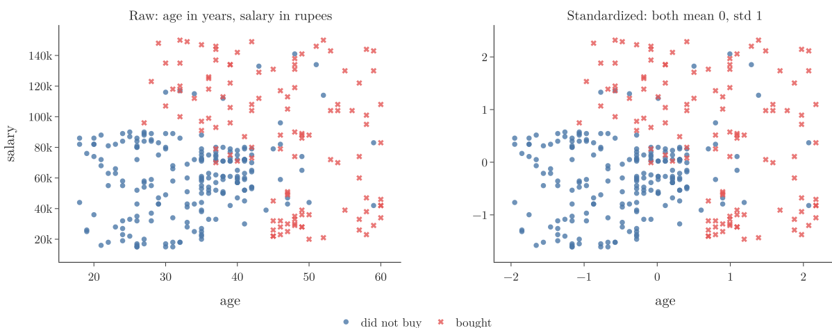
Figure 6: The 320 training users before (left) and after (right) standardizing. Red crosses bought, blue dots did not.
