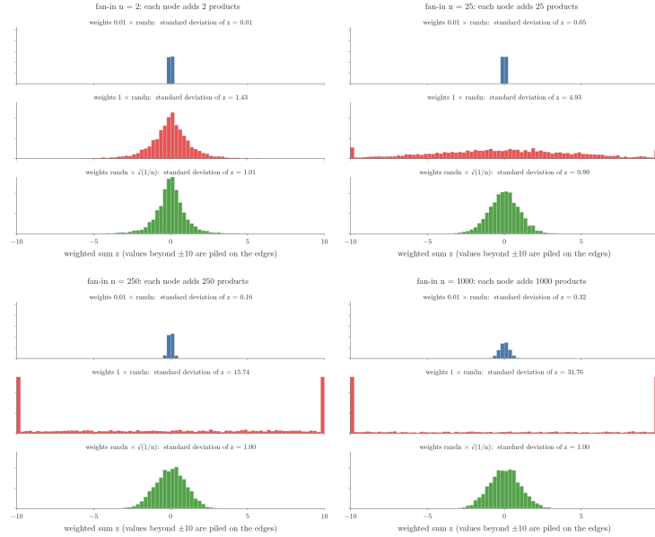
Figure 3: The weighted sum z of one node as its fan-in grows from 2 to 1,000, 4,000 draws per histogram. Top: weights 0.01 \times \text{randn} . Middle: weights 1 \times \text{randn} . Bottom: weights \text{randn} \times \sqrt{1/n}
