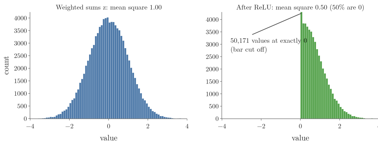
Figure 5: 100,000 weighted sums z , symmetric around 0 (left), and the same values after ReLU (right). The mean square falls from 1.00 to 0.50.
