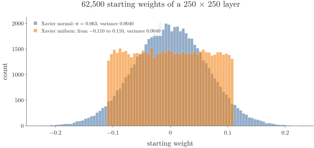
Figure 4: The 62,500 starting weights of a 250 \times 250 layer, drawn with Xavier normal (blue) and Xavier uniform (orange).
