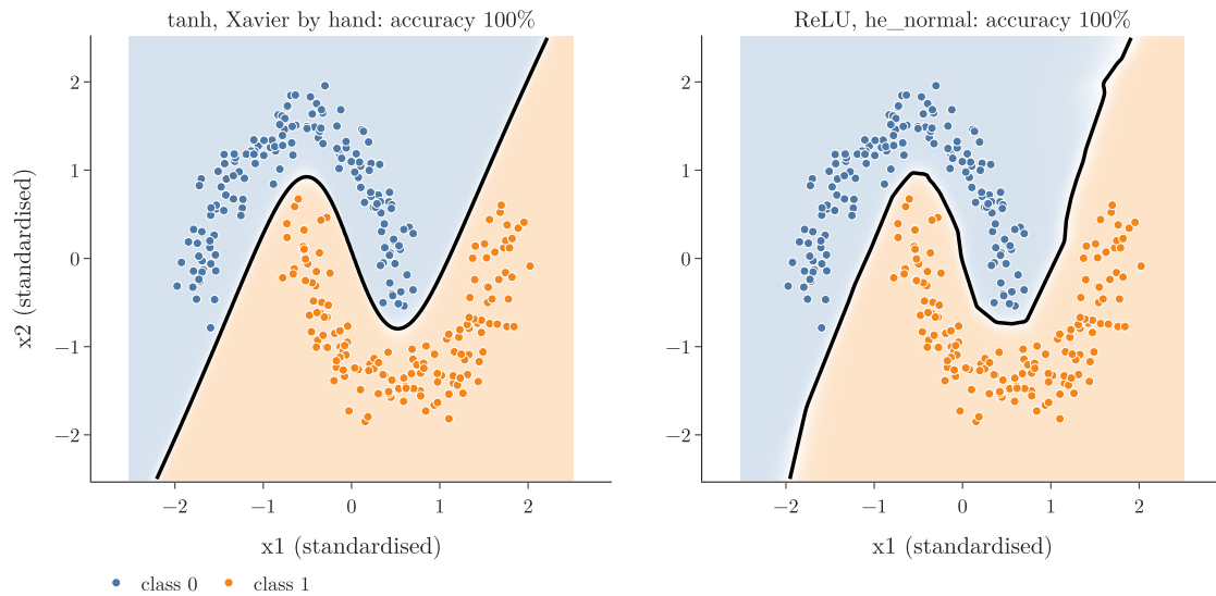
Figure 6: Decision regions after 100 epochs. Left: tanh with Xavier weights set by hand. Right: ReLU with he_normal
