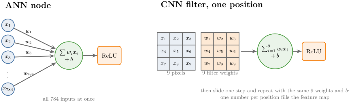
Figure 2: Left: an ANN node takes all 784 inputs, forms a weighted sum, adds its bias and applies ReLU. Right: a 3 \times 3 filter does the same with the 9 pixels under it, then slides to the next position and repeats with the same 9 weights and bias
