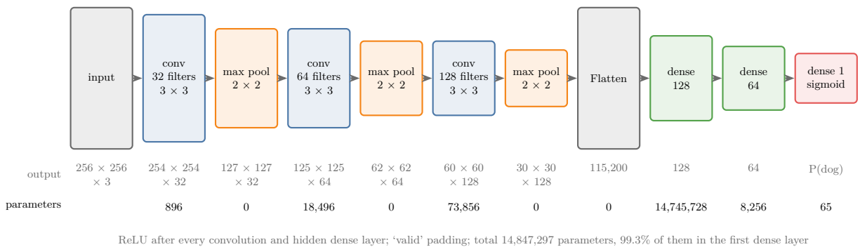
Figure 4: The CNN: three convolution (blue) and max-pooling (orange) blocks, Flatten, and three dense layers. Under each layer: its output size and its number of parameters
