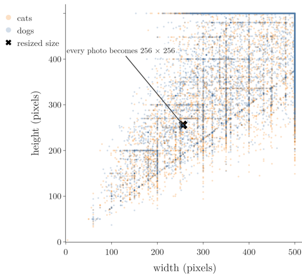
Figure 2: The width and height of all 23,410 photos, one dot each, and the single size every photo is resized to.
