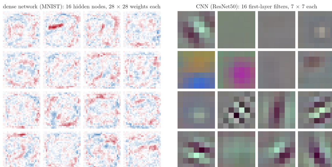
Figure 4: Left: the incoming weights of 16 hidden nodes of a dense network trained on MNIST, each a 28 \times 28 picture (blue positive, red negative). Right: the first 16 first-layer filters of ResNet50. Contrast after 3Blue1Brown, “Gradient descent, how neural networks learn”
