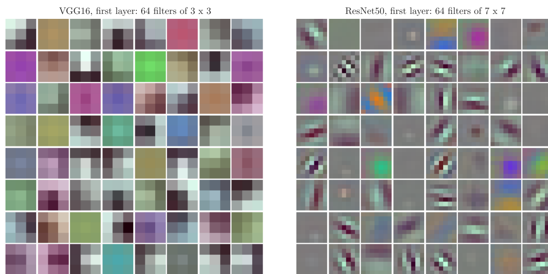
Figure 3: The 64 first-layer filters of VGG16 (left, 3 \times 3 , enlarged) and of ResNet50 (right, 7 \times 7 ), each drawn as a tiny colour image after rescaling
