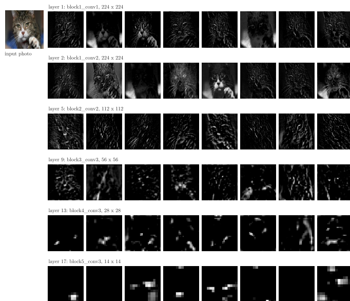
Figure 5: A kitten photo (Wikimedia Commons, David Corby, CC BY 2.5) and the first 8 feature maps it produces at six layers of VGG16. Brighter means a larger value; black means 0
