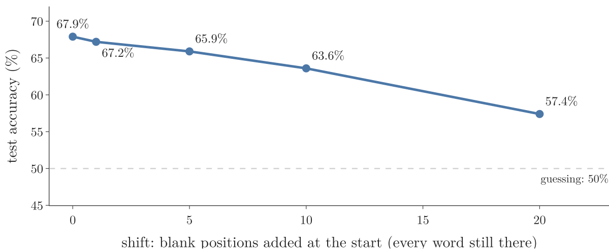
Figure 6: The same test reviews, pushed further to the right. Every word is still there, yet the accuracy falls towards guessing
