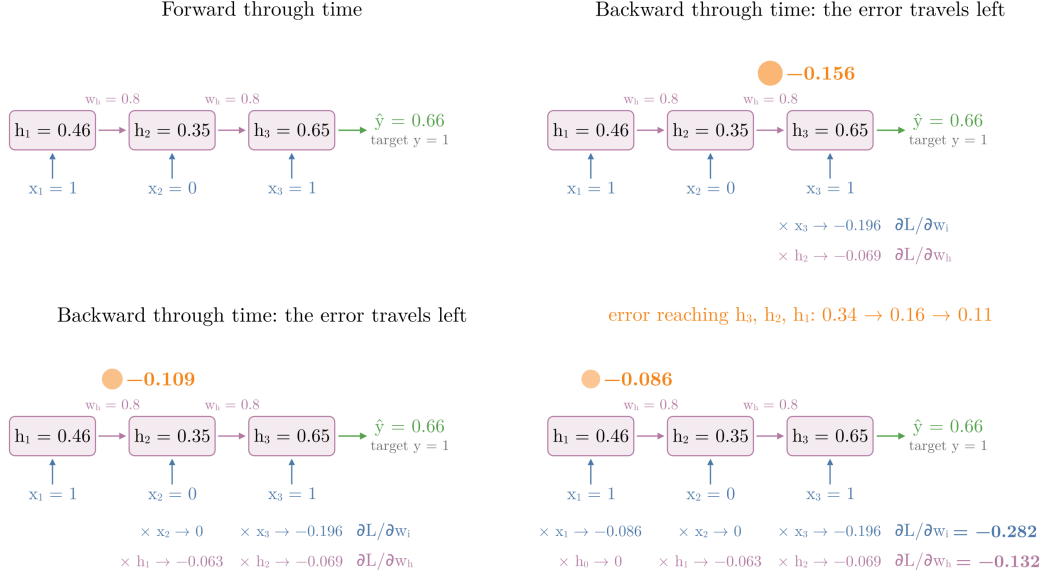
Figure 6: BPTT on the one-node example as one backward walk. The orange disc is the error reaching each hidden state; at each step it is multiplied by the tanh slope, drops one term into \partial L / \partial w_i (times x_t ) and one into \partial L / \partial w_h (times h_{t-1} ), then is multiplied by w_h to reach the step before
