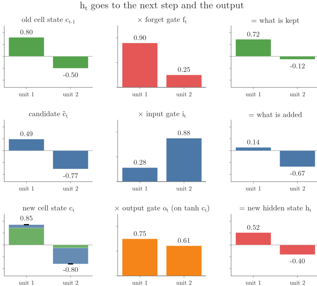
Figure 6: The time step above, one vector per frame. Each row is “value × gate = result”: the forget gate scales the old cell state, the input gate scales the candidate, and the output gate scales \tanh(c_t) . The new cell state is drawn as what is kept (green) plus what is added (blue)
