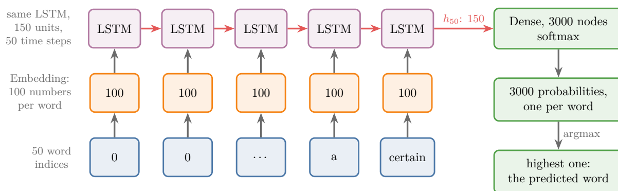
Figure 1: The next-word predictor. The words before the gap become 50 integers (zeros in front), the Embedding layer turns each into 100 numbers, the LSTM reads them one time step at a time, and its last hidden state goes to a softmax layer with one node per vocabulary word. The word with the highest probability is the prediction
