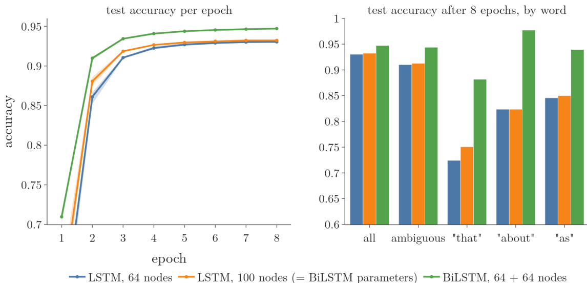
Figure 5: Left: test accuracy per epoch, mean of 3 seeds (band: lowest to highest seed). Right: test accuracy after 8 epochs on all words, on the ambiguous words, and on three ambiguous words separately
