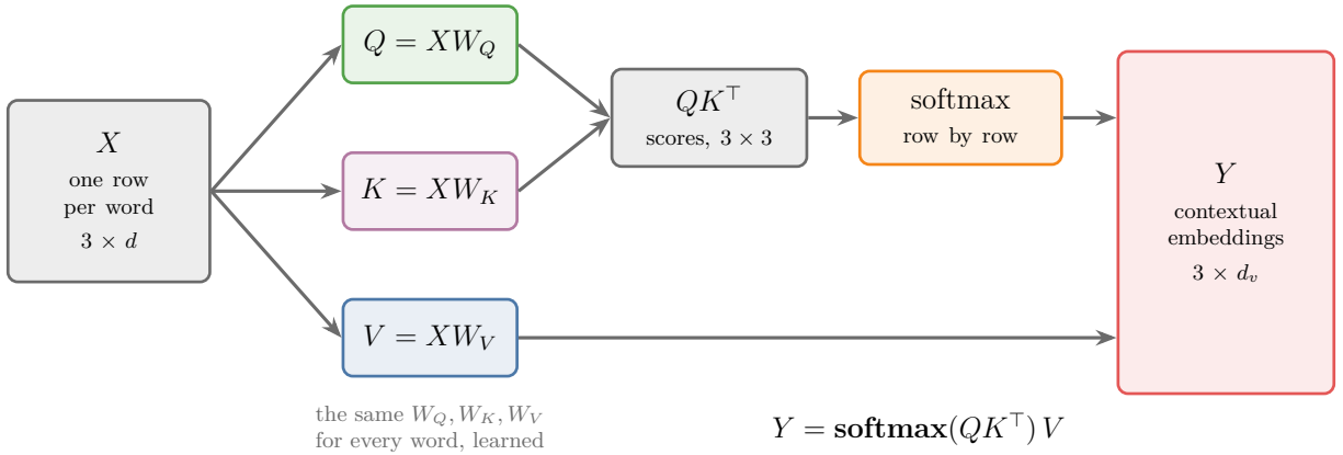
Figure 7: Self-attention with learned matrices, for a whole sentence at once
