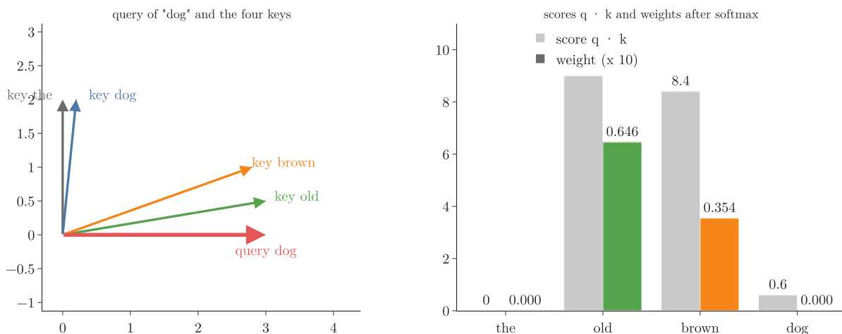
Figure 5: The invented example. Left: the query of “dog” (red) points along the first axis, like the keys of “old” and “brown”; the keys of “the” and “dog” point along the second. Right: the scores and the weights after the softmax
