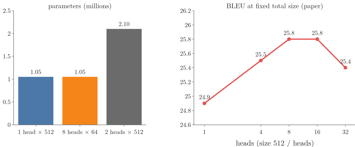
Figure 6: Left: parameters of Keras’ MultiHeadAttention for one head of 512, eight heads of 64 and two full heads of 512 (Notebook). Right: translation quality against the number of heads, with the total size fixed at 512 (Vaswani et al. 2017, Table 3, rows A)
