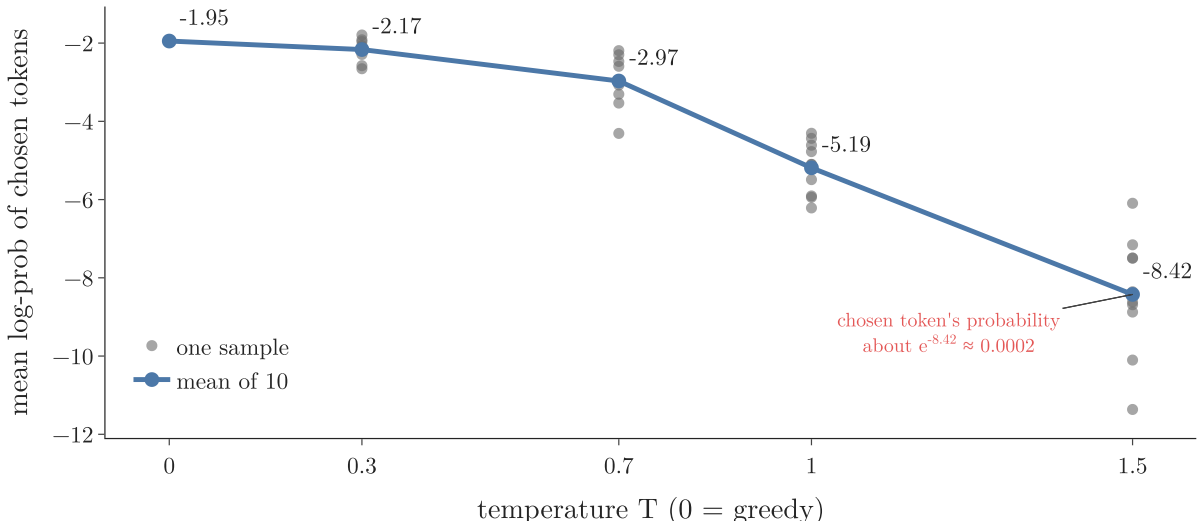
Figure 5: All 50 samples of the table: the mean log-probability of each sample’s 12 chosen tokens (grey dots) and the mean over the 10 samples at each temperature (blue). The spread between samples grows with T too
