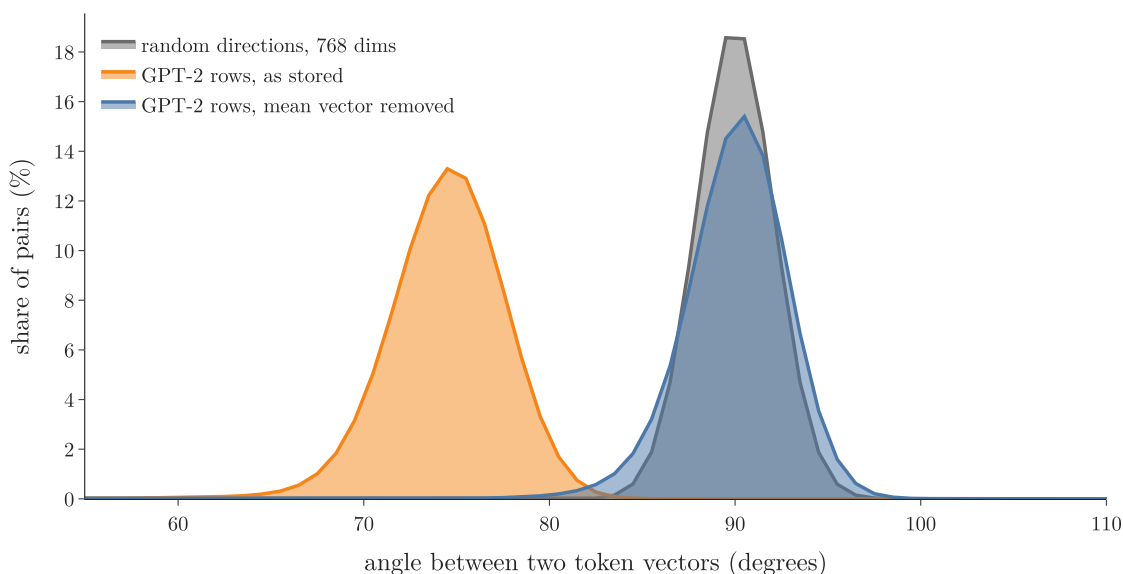
Figure 6: Angles between 3,000 token vectors of GPT-2 small. Orange: as stored. Blue: after subtracting the mean of all 50,257 token vectors. Grey: random directions in 768 dimensions
