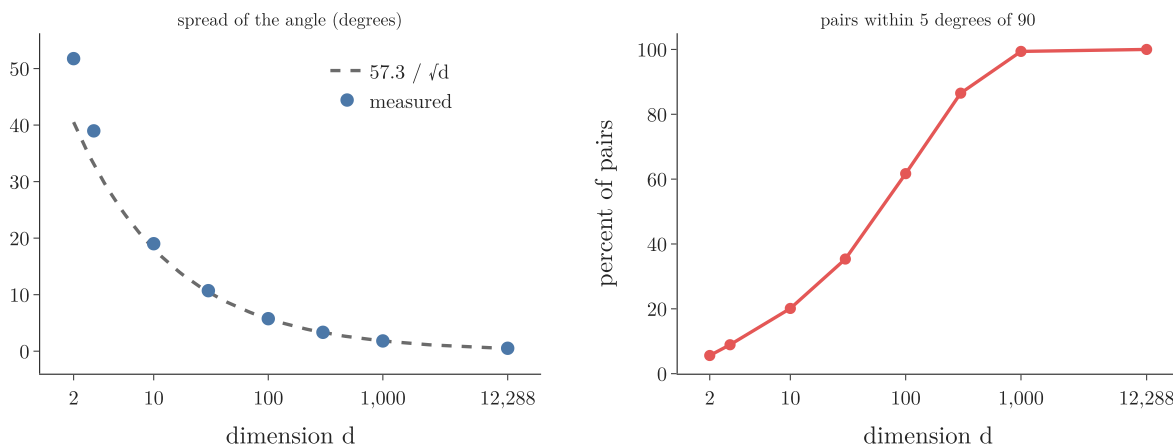
Figure 3: Left: the measured spread of the angle between random directions (dots) against the prediction 57.3/\sqrt{d} (dashed). Right: the share of pairs within 5 degrees of perpendicular rises from 6 percent in 2 dimensions to 100 percent in 12,288
