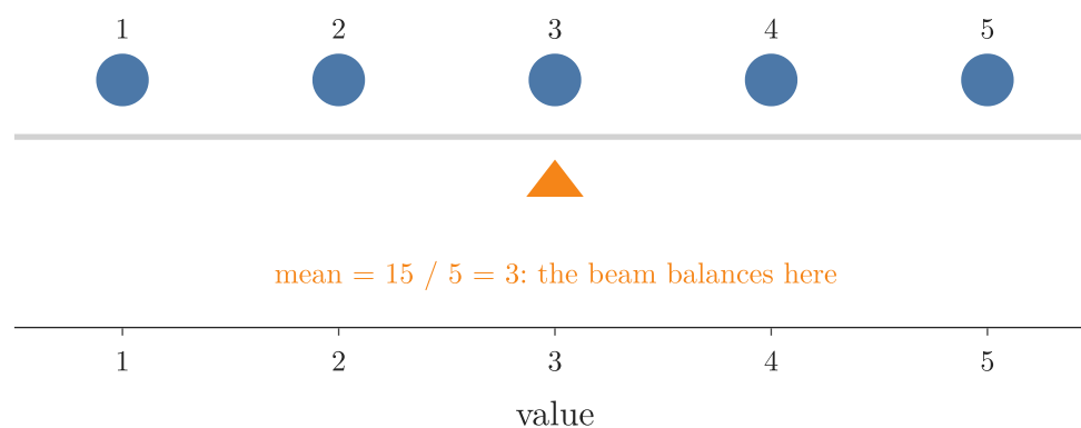
Figure 2: The scores 3, 4, 1, 2, 5 as equal weights on a beam: the mean, 3, is the balance point
