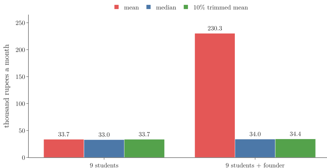
Figure 3: Mean, median and 10% trimmed mean before and after one very high earner joins
