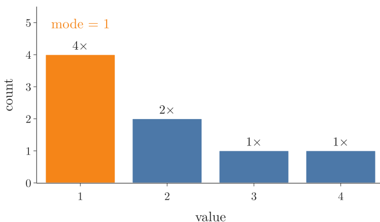
Figure 6: Counting each value of 1, 2, 1, 3, 1, 4, 2, 1: the tallest bar is the mode
