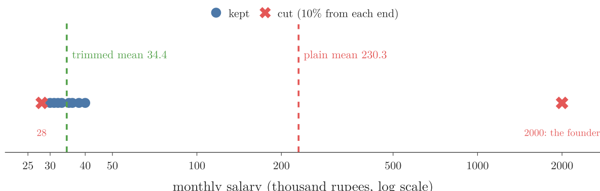
Figure 8: The worked example on a log scale: the 10% trim cuts the lowest salary, 28, and the founder's 2000; the mean of the 8 left is 34.4, while the plain mean of all 10 is 230.3, above every student but one
