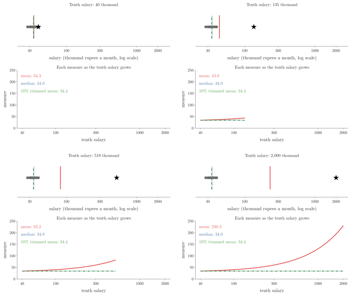
Figure 5: The tenth salary dragged from 40 to 2,000 thousand rupees: the mean follows it up to 230.3, the median stays at 34 and the 10% trimmed mean at 34.4
