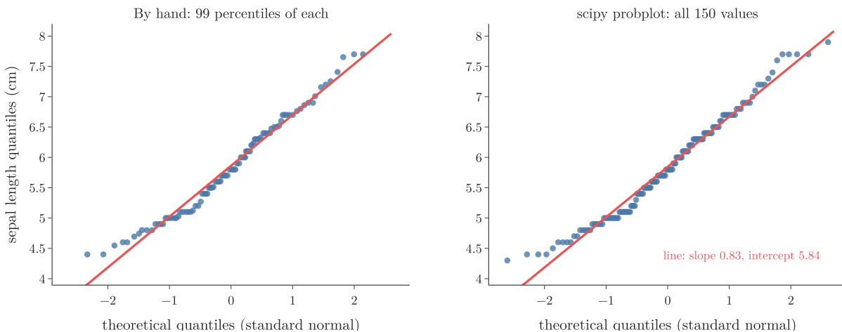
Figure 7: Q-Q plot of the iris sepal lengths against the normal distribution, by hand and with scipy
