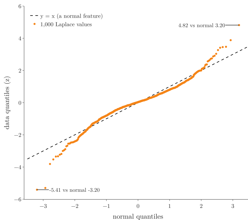
Figure 8: Q-Q plot of 1,000 standardized Laplace values against the normal. The middle follows the dashed line; both ends bend away from it, outwards.
