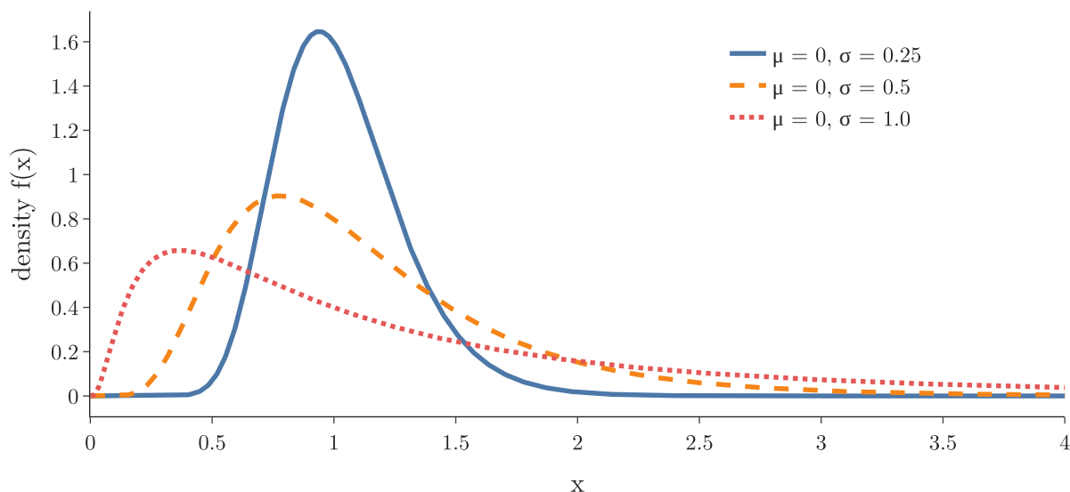
Figure 4: Log-normal PDFs with \mu = 0 and three values of \sigma
