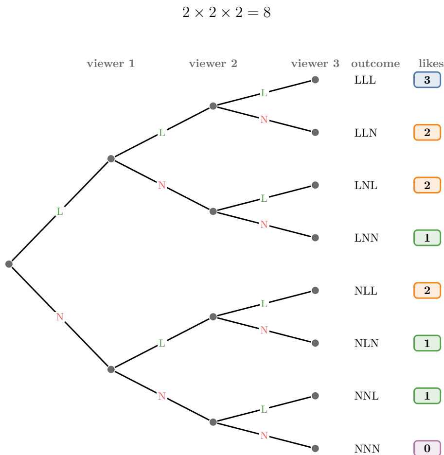
Figure 4: Every outcome for three viewers and the number of likes in each
