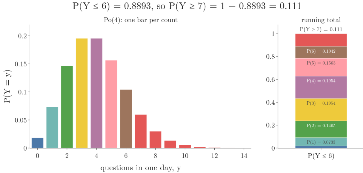
Figure 7: Adding the Po(4) bars for 0 to 6 questions one at a time into a running total, P(Y \leq 6) = 0.8893 . The red remainder up to 1 is P(Y \geq 7) = 0.111 .
