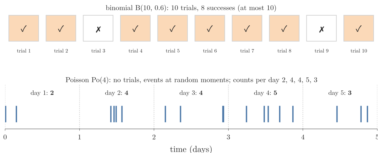
Figure 2: Top: a binomial count, 10 numbered trials with success probability 0.6, here 8 successes. Bottom: a Poisson count, events at random moments with 4 a day on average; the counts per day are 2, 4, 4, 5 and 3. One seeded simulation of each.
