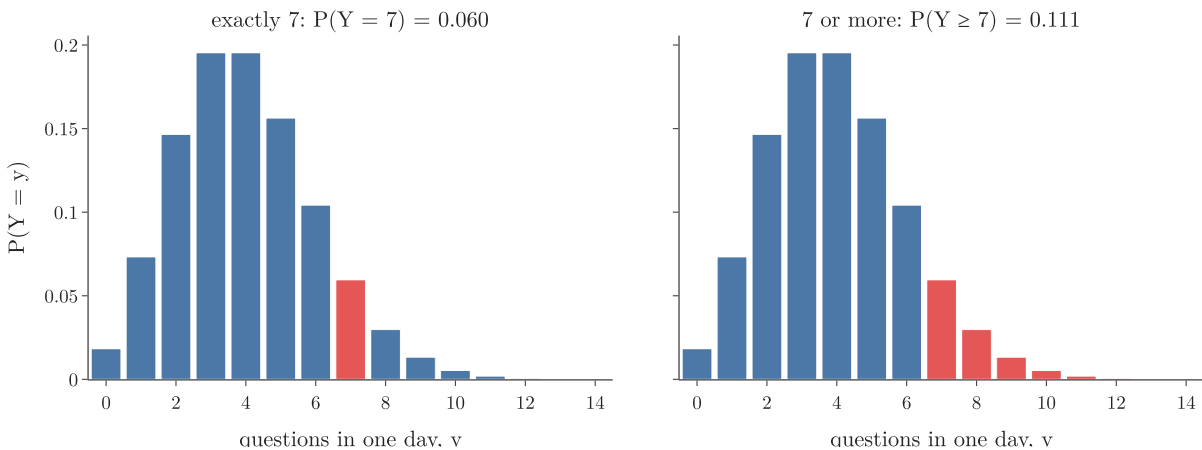
Figure 3: The Poisson PMF with \lambda = 4 : the bar for exactly 7 questions (left) and the bars for 7 or more (right)
