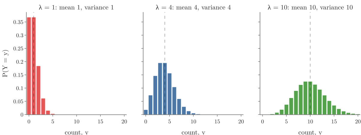
Figure 4: Poisson PMFs for three rates; the dashed line marks the mean \lambda
