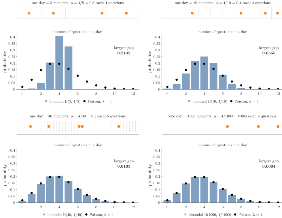
Figure 8: A day cut into n moments, each with a question with probability 4/n (top); the binomial PMF B(n, 4/n) (bars) settles onto the Poisson PMF with \lambda = 4 (dots) as n grows from 5 to 1000
