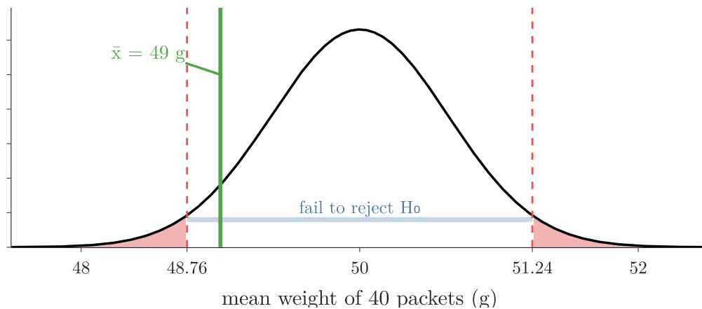
Figure 6: The chips test in grams: sample means between 48.76 g and 51.24 g fail to reject H_0 ; the watchdog's 49 g lies inside
