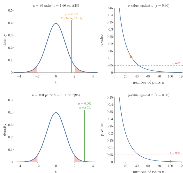
Figure 8: The correlation test for a fixed r = 0.30 as the number of pairs n grows from 10 to 100. Left: the test statistic t (vertical line) on the t-distribution with n - 2 degrees of freedom; the red tails are the 5% rejection region. Right: the p-value against n ; it falls below 0.05 from n = 44 .
