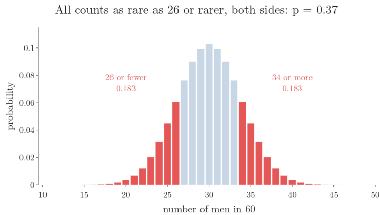
Figure 5: The exact binomial test for 26 men out of 60. Bars: the probability of each count of men if the population is 50/50. Red: the observed count, then every count as rare or rarer on both sides, which add up to p = 0.37 . Idea after StatQuest, “The Binomial Distribution and Test, Clearly Explained!!!”.
