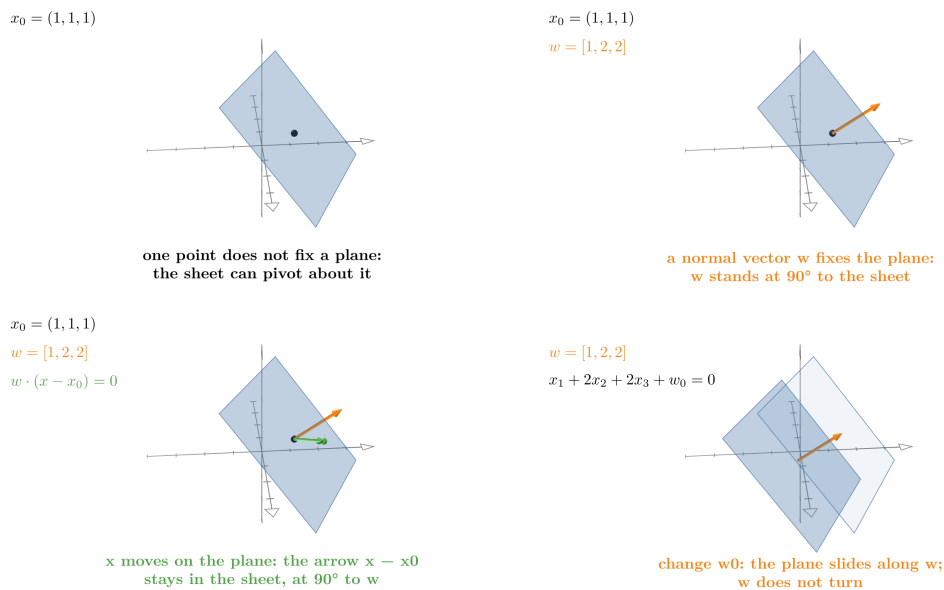
Figure 6: A plane from the point x_0 = (1, 1, 1) and the normal vector w = [1, 2, 2] . The sheet can pivot about one point; the normal vector fixes it; the arrow from x_0 to any point x of the plane stays at 90^\circ to w ; changing w_0 slides the plane along w . Idea after Khan Academy, “Defining a plane in R^3 with a point and normal vector”.
