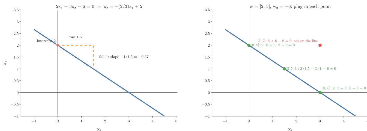
Figure 3: The line 2x_1 + 3x_2 - 6 = 0 . Left: the same line as x_2 = -(2/3)x_1 + 2 , with its slope triangle and intercept 2. Right: [3, 0] , [0, 2] and [1.5, 1] give 0 and lie on the line; [3, 2] gives 6 and does not.
