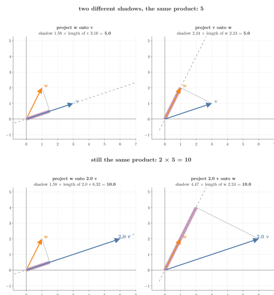
Figure 3: Both views on Section 2's vectors: the shadows differ, the products agree (5), and after stretching v to 2v both give 10
