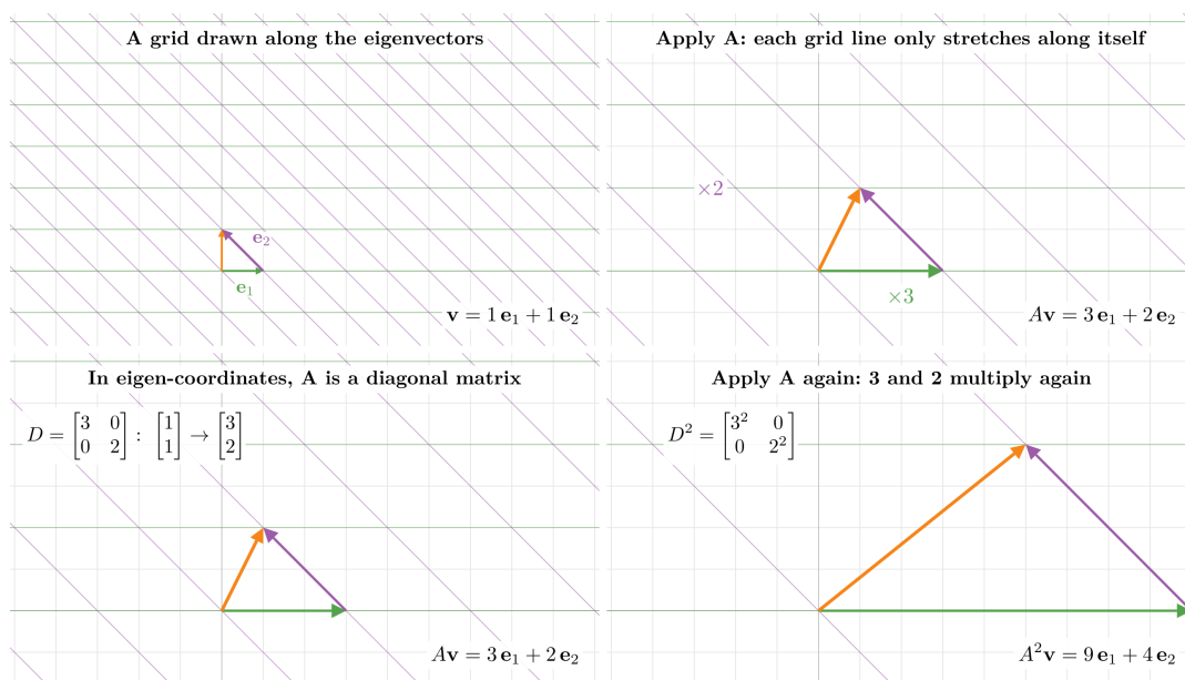
Figure 7: A grid drawn along the eigenvectors \mathbf{e}_1 = [1, 0] and \mathbf{e}_2 = [-1, 1] ; applying A only stretches its lines, so \mathbf{v} = 1 \mathbf{e}_1 + 1 \mathbf{e}_2 lands on 3 \mathbf{e}_1 + 2 \mathbf{e}_2 , then 9 \mathbf{e}_1 + 4 \mathbf{e}_2
