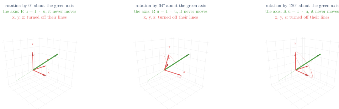
Figure 3: A rotation about the axis through [1, 1, 1] , from 0 to 120 degrees. Red: the basis vectors x , y and z , turned off their lines. Green: the axis, an eigenvector with eigenvalue 1, which never moves.
