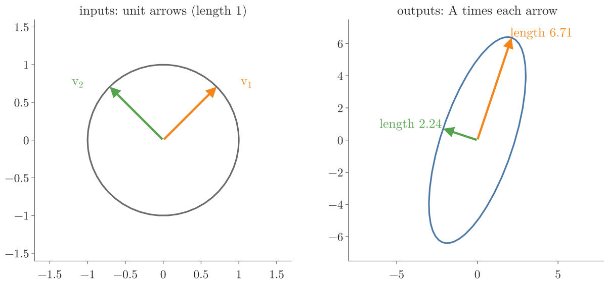
Figure 6: Left: arrows of length 1 end on the unit circle; two of them, \mathbf{v}_1 and \mathbf{v}_2 , are drawn. Right: the matrix A sends the circle to an ellipse; \mathbf{v}_1 comes out longest, 6.71, and \mathbf{v}_2 shortest, 2.24
