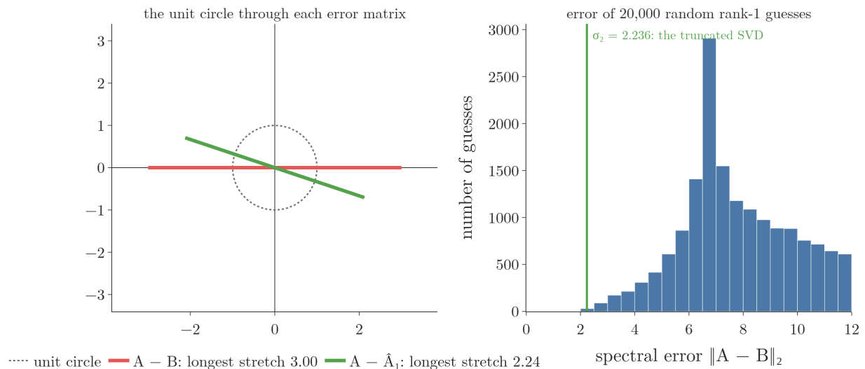
Figure 7: Eckart–Young on the 2 \times 2 example. Left: the unit circle (dotted) sent through the error of the truncated SVD (green, longest stretch 2.24) and through the error of the other guess B (red, longest stretch 3). Right: the spectral errors of 20,000 random rank-1 matrices; none falls below \sigma_2 = 2.236 (green line).
