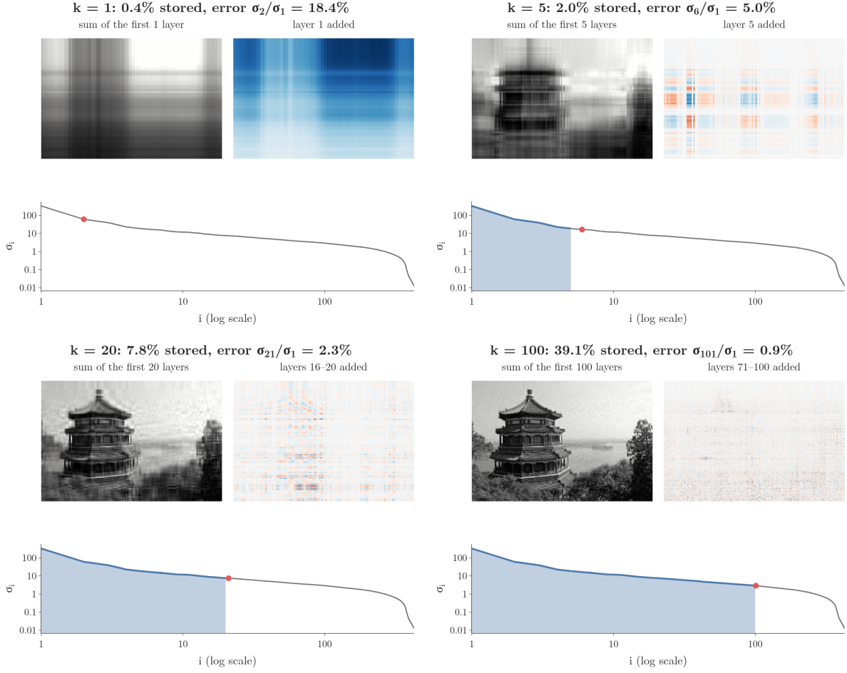
Figure 8: The photo rebuilt layer by layer, k = 1 to 100: the sum of the first k layers (left), the layers just added (right, blue positive, red negative) and the singular values kept so far (filled)
