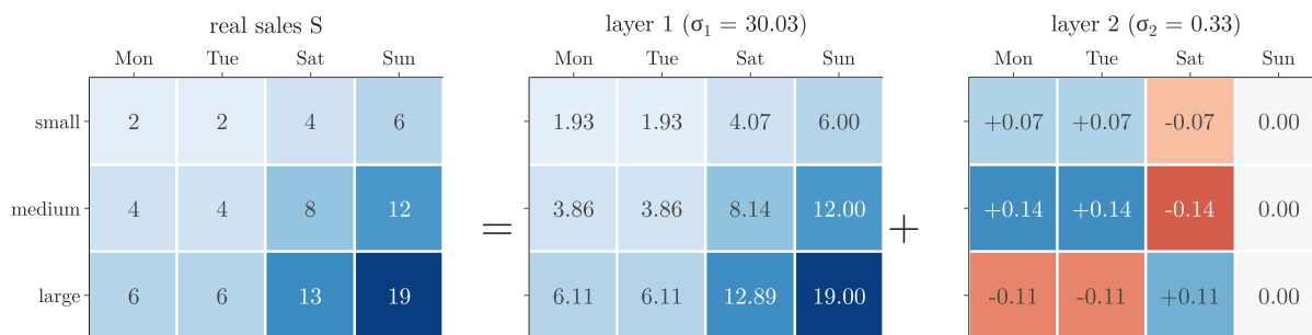
Figure 3: The real sales table S (left) split by the SVD into layer 1 (middle), a column times a row scaled by \sigma_1 = 30.03 , plus layer 2 (right), a much smaller column times a row scaled by \sigma_2 = 0.33 . Blue is positive, red negative
