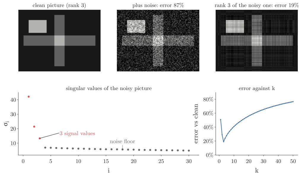
Figure 10: Noise reduction: a rank-3 picture, the same with noise, and the rank-3 approximation of the noisy one
