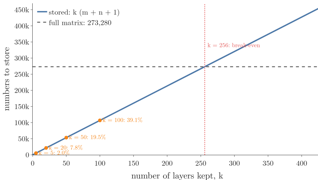
Figure 5: The numbers stored for a rank- k approximation of the 427 \times 640 photo, k(m + n + 1) , against the 273,280 numbers of the full matrix. k = 20 needs 7.8%; from k = 256 on, the layers cost more than the matrix.
