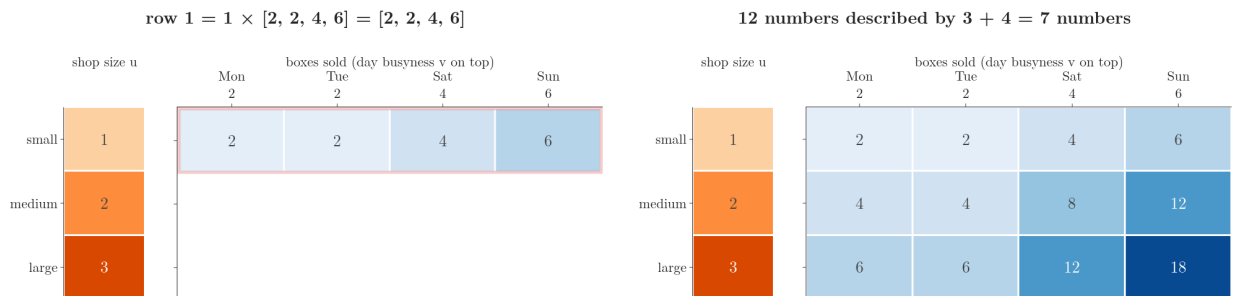
Figure 2: The plan table built row by row: each row is the branch size (orange, left) times the row of day busyness [2, 2, 4, 6] (top). The finished table has 12 entries but is fully described by 3 + 4 = 7 numbers
