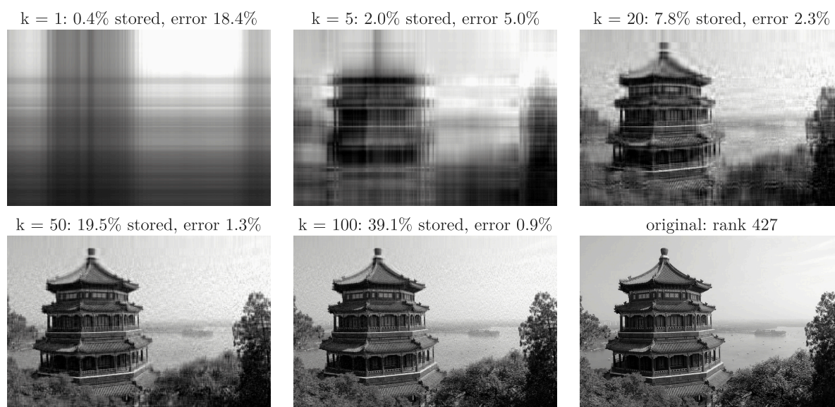
Figure 1: A 427 \times 640 photo rebuilt from its first k layers: “stored” is the share of numbers kept, “error” is the size of the biggest dropped layer relative to the biggest kept one
