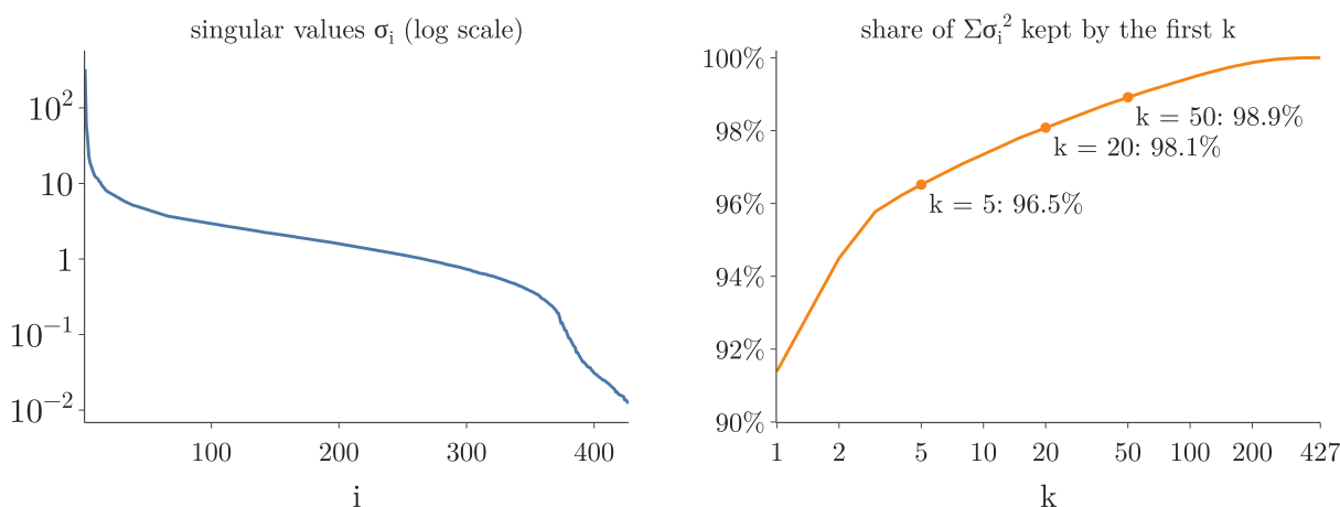
Figure 9: Singular values of the photo, and the share of \sum \sigma_i^2 kept by the first k
