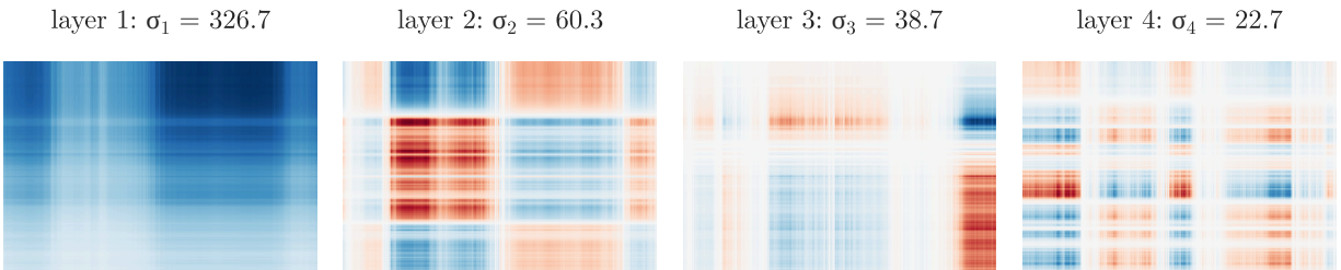
Figure 4: The first four layers \sigma_i \mathbf{u}_i \mathbf{v}_i^\top of the photo: blue positive, red negative, white zero
