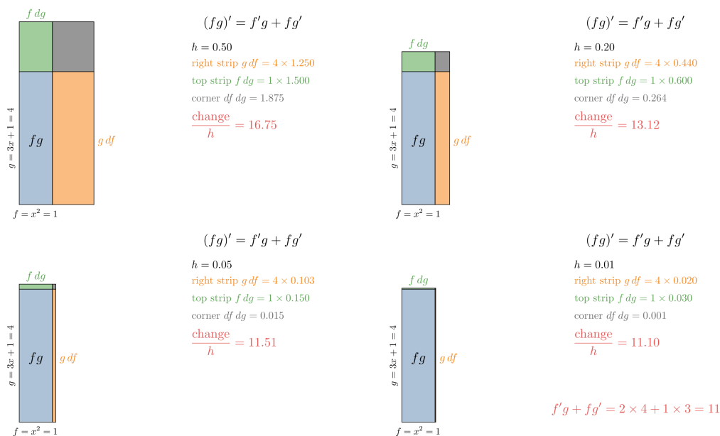
Figure 7: The product fg as the area of a rectangle with sides f = x^2 and g = 3x + 1 (1 by 4 at x = 1 ). Nudging x by h adds a right strip gdf , a top strip fdg and a tiny corner; the change divided by h settles at 11
