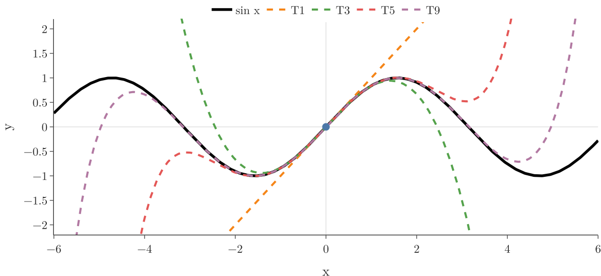
Figure 11: Taylor polynomials of \sin x around x_0 = 0 (blue dot): each higher degree follows the curve over a wider range
