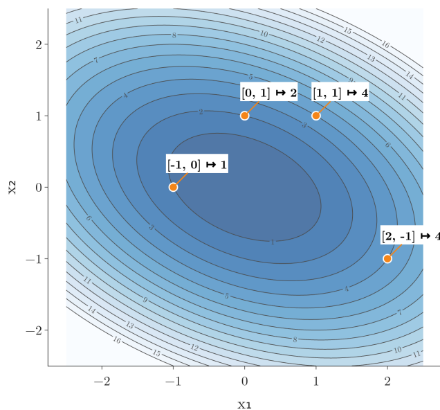
Figure 3: The running example on a contour map, with four input vectors and the single number the function returns for each. [1, 1] and [2, -1] both give 4 and lie on the same contour line.
