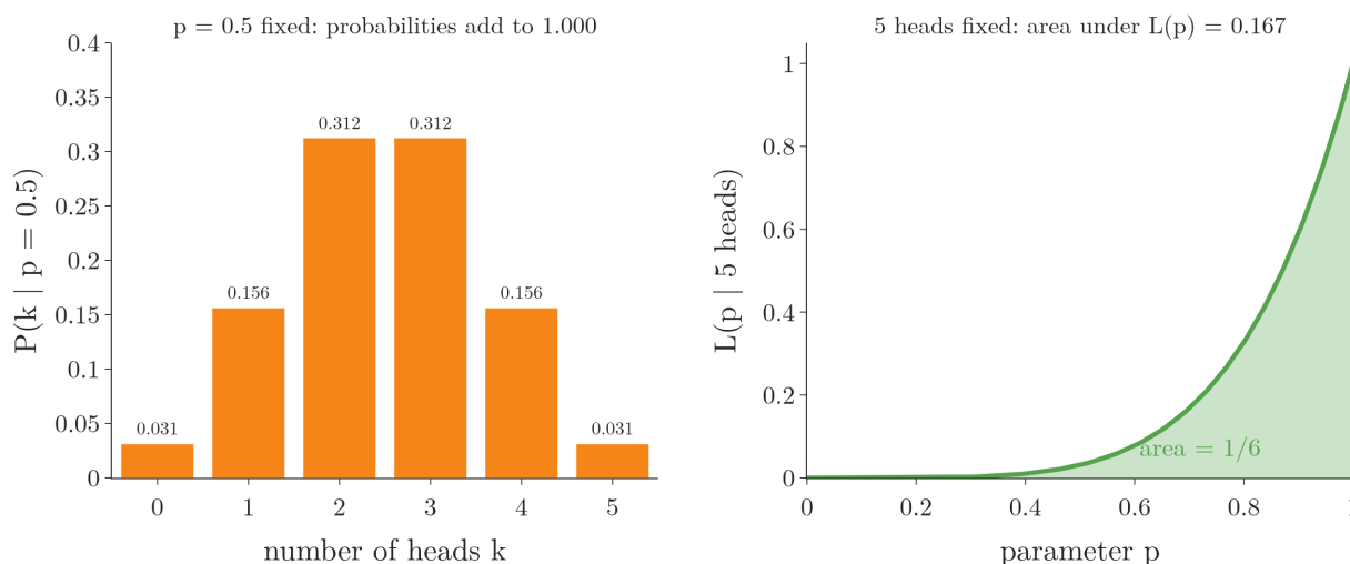
Figure 7: Left: with p = 0.5 fixed, the probabilities of 0 to 5 heads add up to 1. Right: with five heads fixed, the area under the likelihood L(p) = p^5 is 1/6 .
