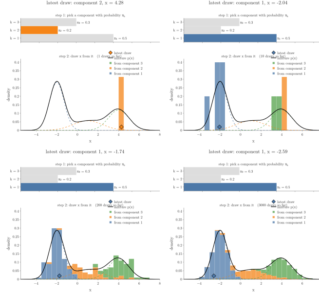
Figure 4: Sampling from a mixture in two steps. Top: pick one of three normal curves with probabilities 0.5, 0.2 and 0.3. Bottom: draw a value from the picked curve. As the draws pile up, their histogram takes the shape of the mixture density (black)
