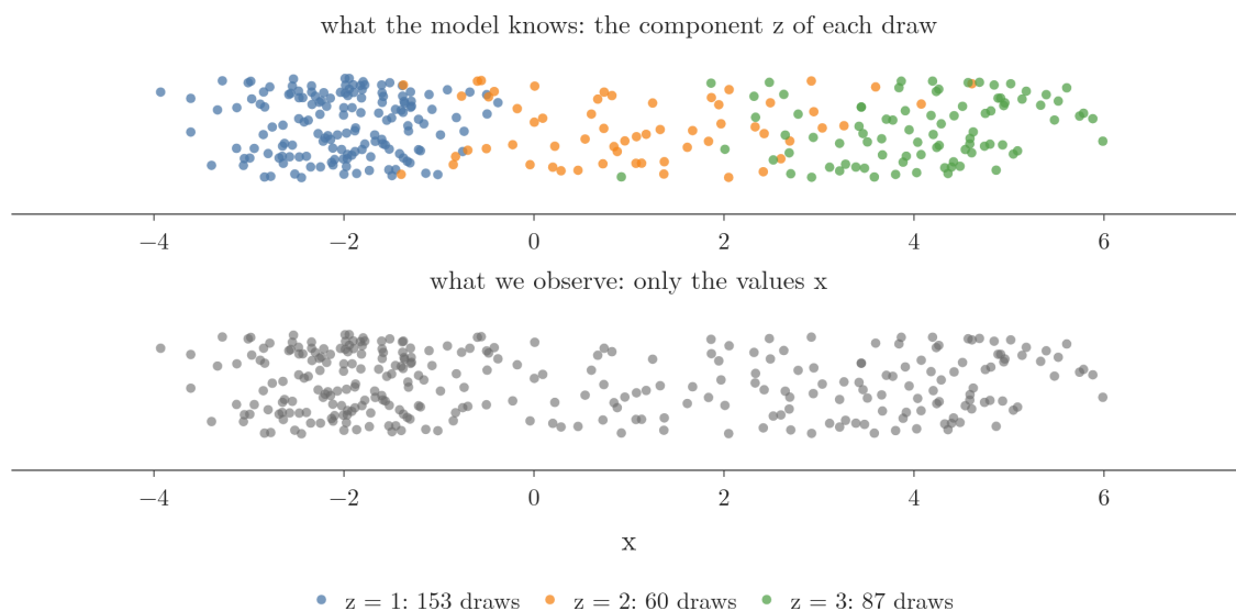
Figure 5: 300 draws from the mixture of Figure 6. Top: coloured by the component z that produced each draw, which the model knows. Bottom: the same draws as we observe them, with z lost.
