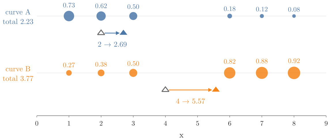
Figure 3: The update on the six points. Row A and row B: each point is as large as its share of that curve (label). Each centre moves from its start (hollow triangle) to the share-weighted average (filled triangle)
