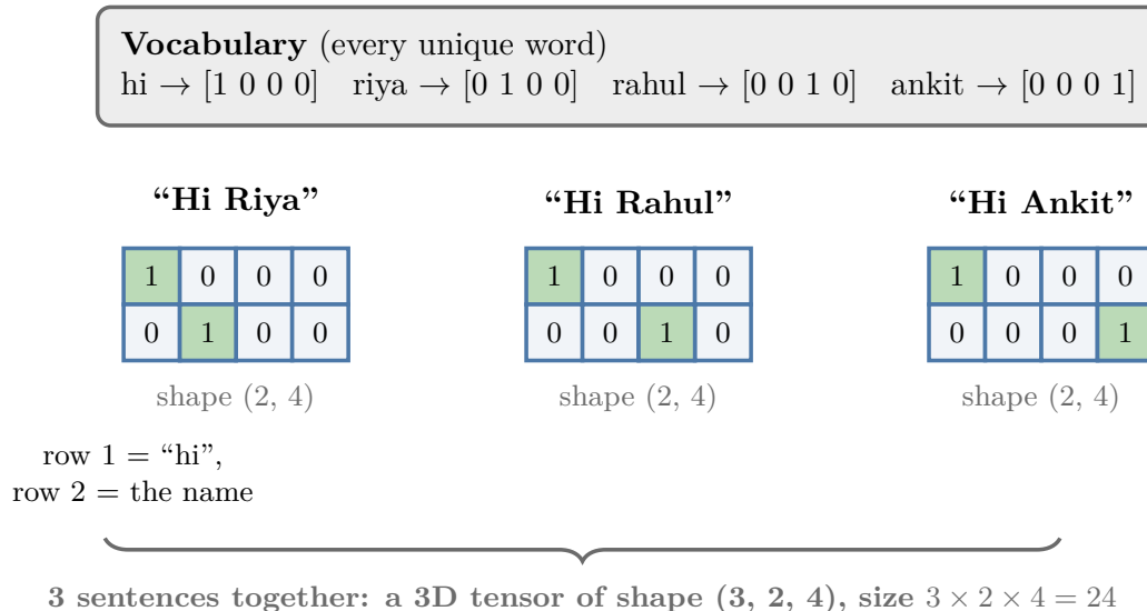
Figure 7: Sentences as a 3D tensor
