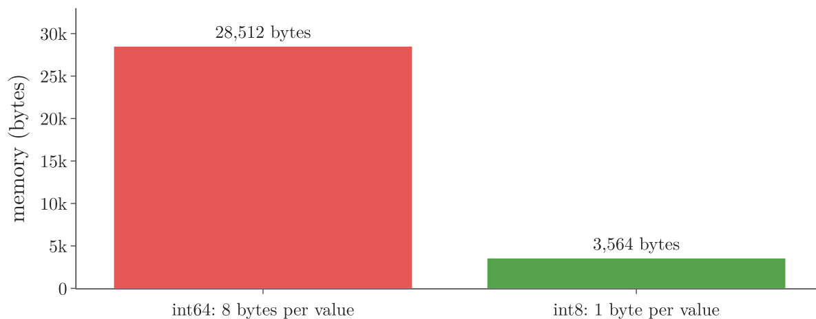
Figure 3: The four small-number columns stored as int64 and as int8, measured with pandas: 28,512 bytes against 3,564
