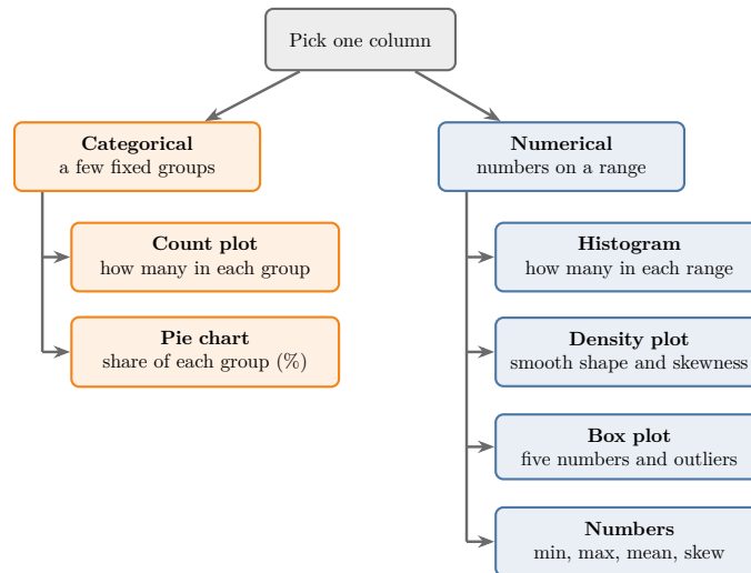
Figure 1: Which graphs to draw for one column, by its type
