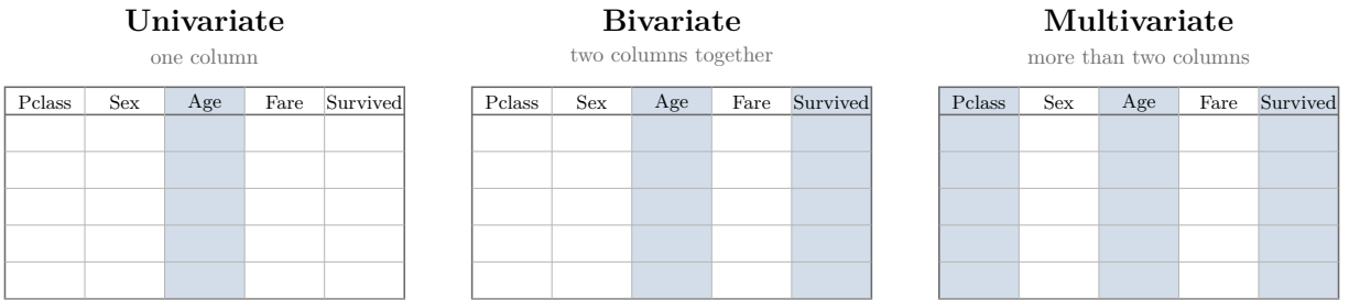
Figure 2: The three levels of analysis: the shaded columns are studied together
