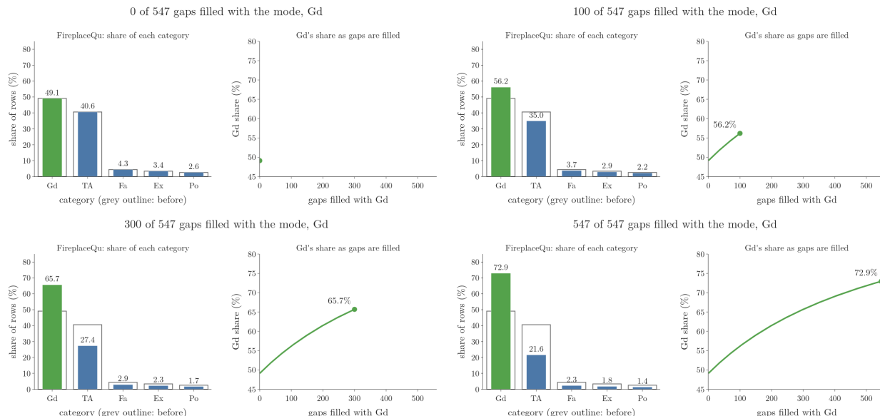
Figure 2: Mode imputation gap by gap on FireplaceQu: each filled gap adds to Gd, so Gd’s share rises from 49.1% to 72.9% and every other category shrinks
