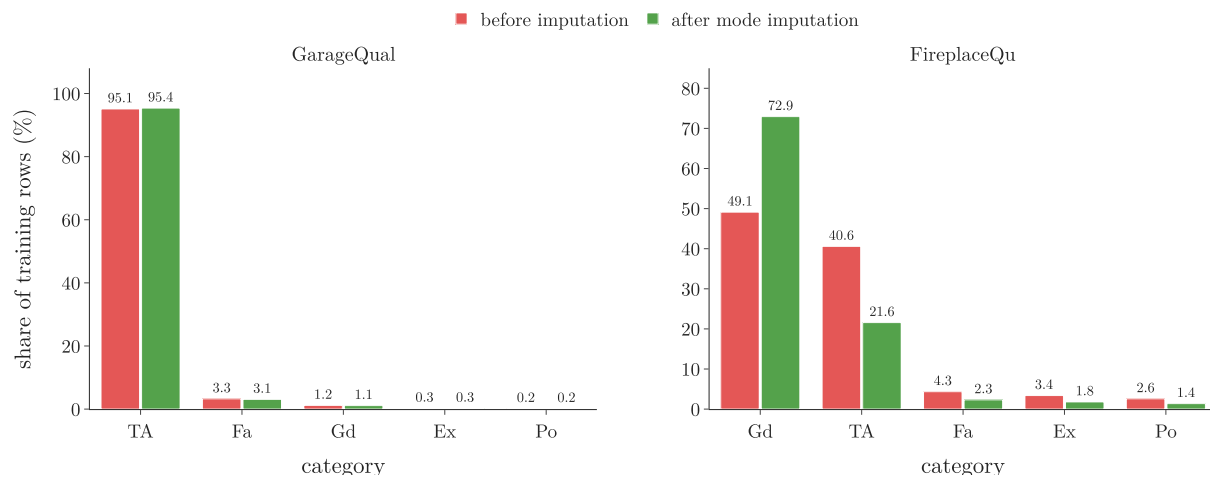
Figure 4: Category shares in the training set before and after mode imputation: GarageQual barely moves, while Gd in FireplaceQu jumps from 49.1% to 72.9%
