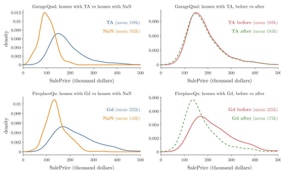
Figure 5: Sale prices as density curves. Left: houses in the most frequent category against houses with a gap. Right: the most frequent category before and after imputation
