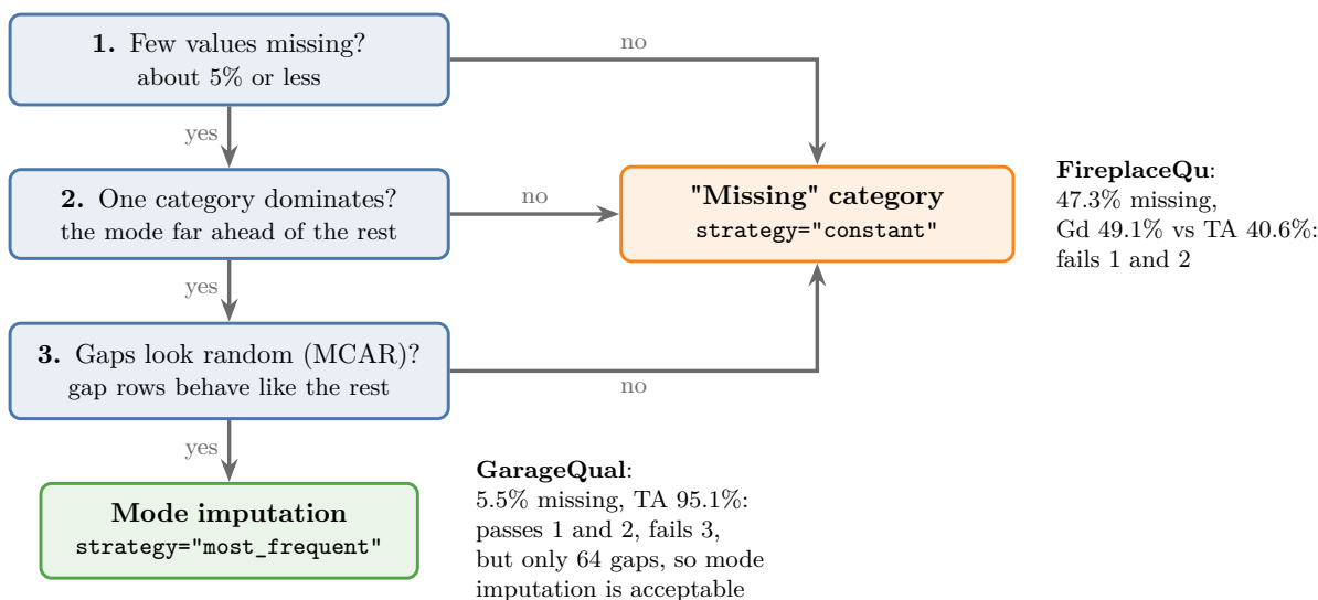
Figure 7: Choosing the imputer: three questions in order, with the two house-price columns placed where they end
