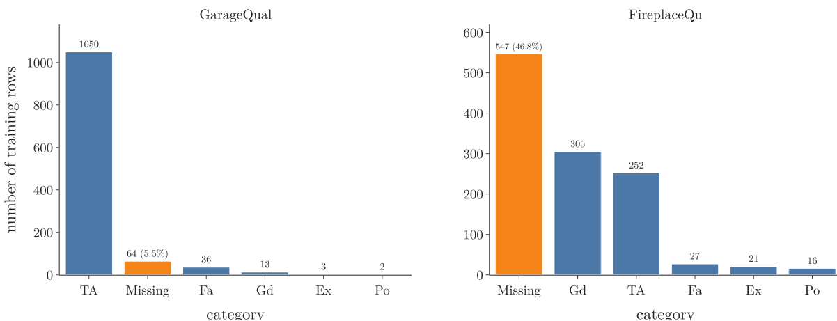
Figure 6: Category counts in the training set after adding the category “Missing” (orange); every other count is unchanged
