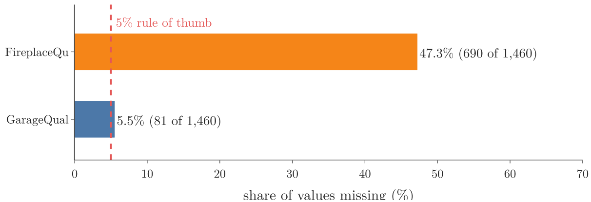
Figure 3: Share of missing values in each column, against the 5% rule of thumb for mode imputation
